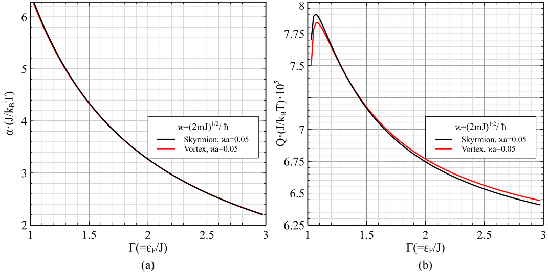
FIG. 1. (a) Seebeck coefficient and (b) Nernst coefficient for skyrmion/vortex sizes \varkappa a = 0.05
