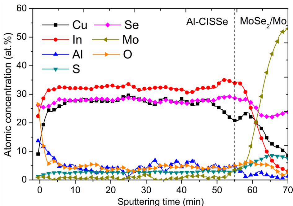
Figure 3. AES depth profiling of Al-CISSe. The bulk Al-CISSe film has average ratios of \text{Cu}/(\text{Al}+\text{In}) : 0.75, \text{Al}/(\text{Al}+\text{In}) : 0.12, \text{Se}/(\text{S}+\text{Se}) : 0.91, as estimated from the AES spectra (sputtering time of 5 to 50 min).
