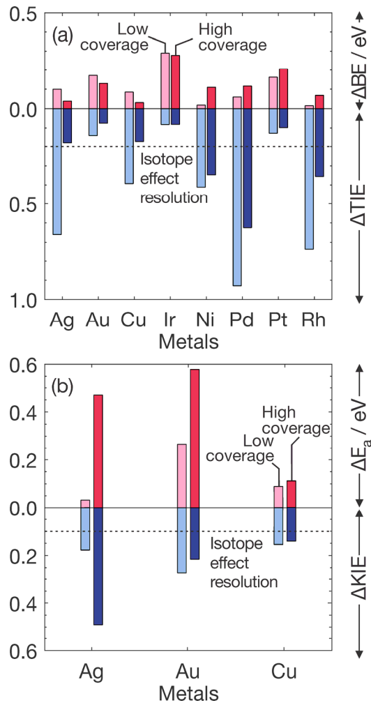
Figure 10 Structure-sensitivity of TIEs and KIEs for dissociative adsorption of H 2 /D 2 on transition metal surfaces. (a) Maximum variation in TIEs ( \Delta TIE ) and BEs ( \Delta BE ) across the (111), (100), and (211) facets of various metals at low and high coverage. Re, Ru, Fe, and Co are not shown as only close-packed surfaces were considered for these metals. (b) Maximum variation in KIEs ( \Delta KIE ) and activation energies ( \Delta E_a ) across the (111), (100), and (211) facets of Ag, Au, and Cu at low and high coverage. Isotope effects are evaluated at 623 K and 0.1 atm H 2 /D 2 pressure. Dashed lines mark the typical resolution of isotope effect measurements (0.1).
