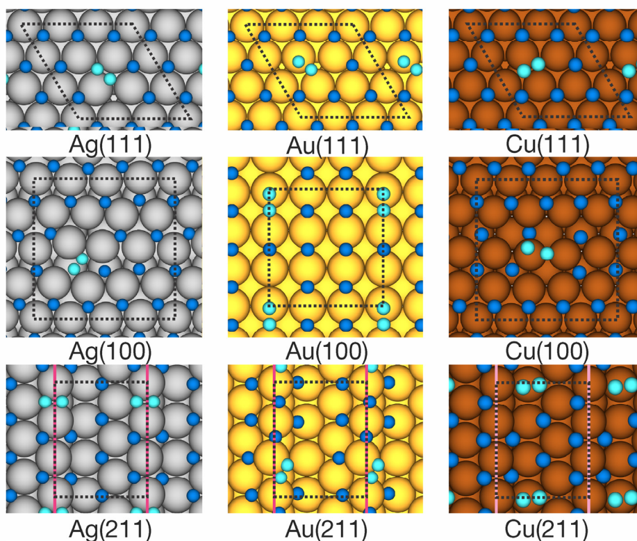
Figure 7 Top views of most stable high-coverage transition state structures for H 2 /D 2 dissociative adsorption on the fcc (111), fcc (100), and fcc (211) surfaces of Ag, Au, and Cu. Pink lines mark the step edges of the (211) surfaces. The unit cell is marked by dashed lines. Color code: grey – Ag, yellow – Au, brown – Cu, blue – spectator H, cyan – dissociating H 2 molecule.
