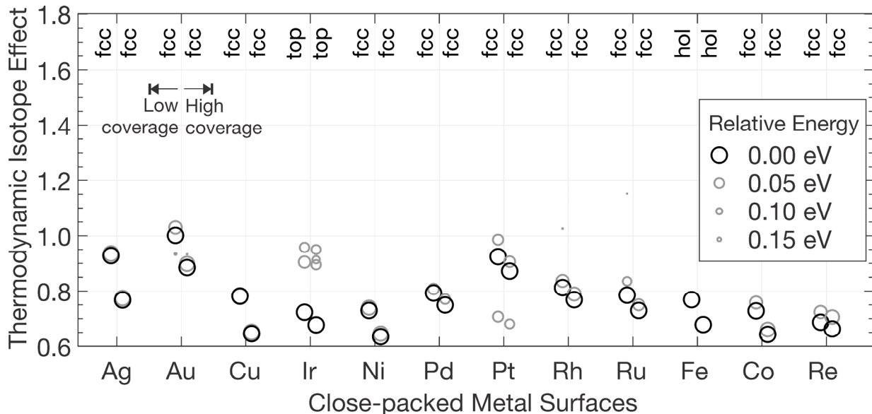
Figure 2 Calculated thermodynamic isotope effects (TIEs) for \text{H}_2/\text{D}_2 dissociative adsorption on close-packed surfaces. Circles mark the TIE for each calculated structure in Table 1. For each metal, the left-most data points correspond to the low coverage (1/9 ML) TIEs; the right-most data points correspond to the high coverage (1 ML) TIEs. Larger circles reflect more stable structures; the circles sizes are based on a Boltzmann distribution at 623 K. The most stable structures for each surface and coverage are highlighted in black and are labelled by their names at the top x -axis. All TIEs are evaluated at 623 K and 0.1 atm \text{H}_2/\text{D}_2 pressure.
