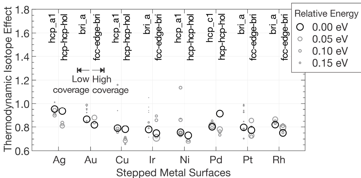
Figure 6 Calculated thermodynamic isotope effects (TIEs) for \text{H}_2/\text{D}_2 dissociative adsorption on stepped surfaces. Circles mark the TIE for each calculated structure in Table 3. For each metal, the left-most data points correspond to the low coverage (1/9 ML) TIEs; the right-most data points correspond to the high coverage (1 ML) TIEs. Larger circles reflect more stable structures; the circles sizes are based on a Boltzmann distribution at 623 K. The most stable structures for each surface and coverage are highlighted in black and are labelled by their names at the top x -axis. All TIEs are evaluated at 623 K and 0.1 atm \text{H}_2/\text{D}_2 pressure.
