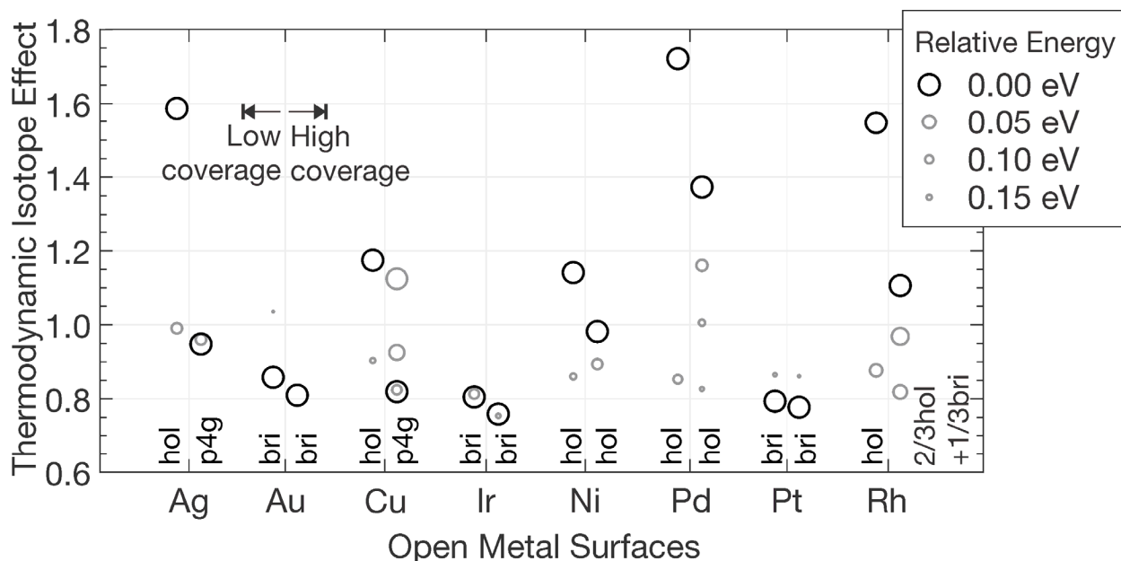
Figure 4 Calculated thermodynamic isotope effects (TIEs) for H_2/D_2 dissociative adsorption on open surfaces. Circles mark the TIE for each calculated structure in Table 2. For each metal, the left-most data points correspond to the low coverage (1/9 ML) TIEs; the right-most data points correspond to the high coverage (1 ML) TIEs. Larger circles reflect more stable structures; the circles sizes are based on a Boltzmann distribution at 623 K. The most stable structures for each surface and coverage are highlighted in black and are labelled by their names at the top x -axis. All TIEs are evaluated at 623 K and 0.1 atm H_2/D_2 pressure.
