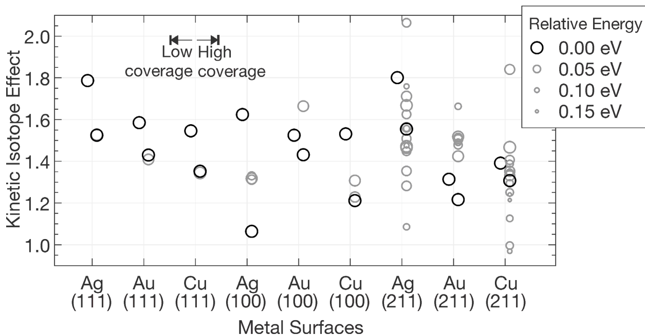
Figure 8 Calculated kinetic isotope effects (KIEs) for \text{H}_2/\text{D}_2 dissociative adsorption on Ag, Au, and Cu surfaces. For each metal, the left-most data point corresponds to the low coverage (2/9 ML) KIE; the right-most data point corresponds to the high coverage (1 ML) KIE. Circles mark the KIE for each calculated structure in Table 4. Larger circles reflect more stable structures; the circles sizes are based on a Boltzmann distribution at 623 K. The most stable structures for each surface and coverage are highlighted in black and correspond to entry numbers of 1 for each surface and coverage in Table 4. All KIEs are evaluated at 623 K and 0.1 atm \text{H}_2/\text{D}_2 pressure.
