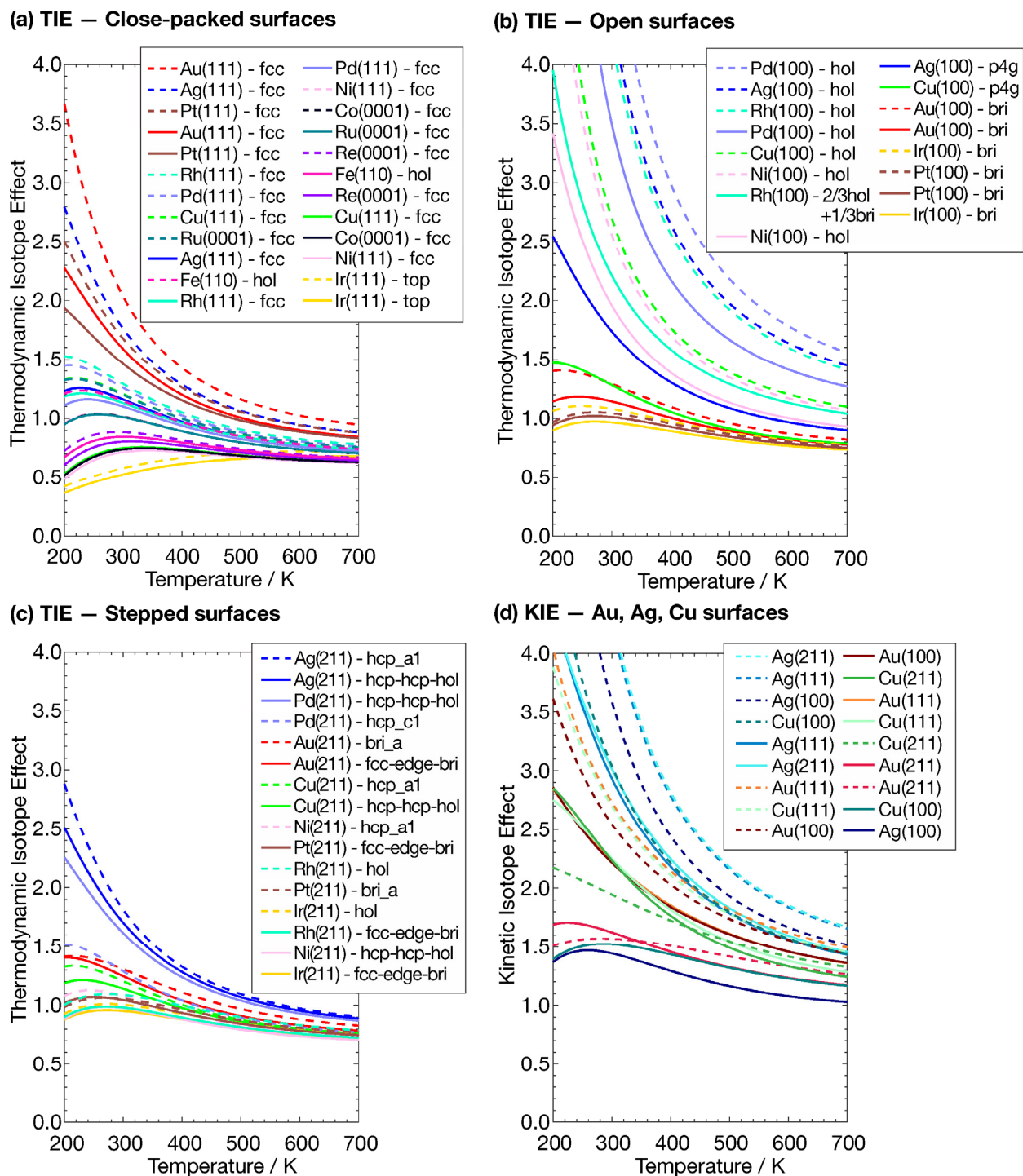
Figure 9 Temperature dependence of (a-c) thermodynamic isotope effects (TIEs) for the most stable adsorption structures on (a) close-packed, (b) open, and (c) stepped transition metal surfaces; and (d) kinetic isotope effects (KIEs) on close-packed, open, and stepped surfaces of Ag, Au, and Cu. Dashed and full lines represent low coverage and high coverage structures respectively.
