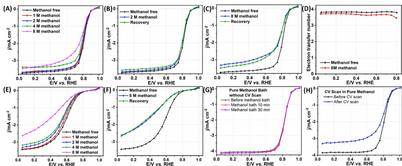
Fig. 1. ORR polarization plots of the Fe-N-C catalysts in O 2 saturated 0.5 M H 2 SO 4 aqueous solution containing different methanol concentrations (A) and their selected rinse recovery polarization plots obtained by transferring the electrode back in a methanol-free electrolyte (B and C) with a rotating rate of 900 rpm. (D) Electron transfer number of Fe-N-C catalysts in O 2 -saturated 0.5 M H 2 SO 4 electrolyte without and within 8 M methanol, respectively. ORR polarization plots of the ZIF-8-derived N-C catalysts in O 2 -saturated 0.5 M H 2 SO 4 aqueous solution containing different methanol concentrations (E) and the selected recovery in methanol-free O 2 -saturated 0.5 M H 2 SO 4 electrolyte (F) with a rotating rate of 900 rpm. ORR polarization plots of the Fe-N-C catalysts in O 2 saturated 0.5 M H 2 SO 4 with rotating speed of 900 rpm (G) after pure methanol bath without CV scan and (H) after pure methanol bath with CV scan (0-1.0 V, 20 cycles).
