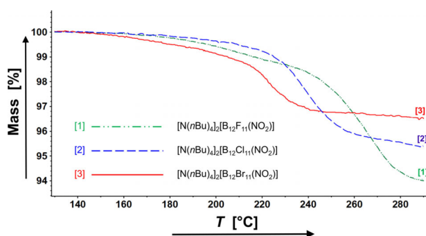
Figure 6. Thermogravimetric analyses of [N( n Bu) 4 ] 2 [B 12 X 11 (NO 2 )] (X = F, Cl, Br) with a heating rate of 5 K min −1 .
