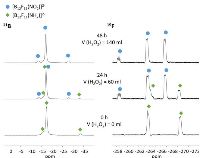
Figure 1. ^{11}\text{B} (left) and ^{19}\text{F} NMR spectra (right) of the oxidation of [\text{K}[\text{B}_{12}\text{F}_{11}(\text{NH}_3)]]^- with \text{H}_2\text{O}_2 over time. Resonances of the starting material [\text{B}_{12}\text{F}_{11}(\text{NH}_3)]^- are marked with green diamonds and those from the product [\text{B}_{12}\text{F}_{11}(\text{NO}_2)]^{2-} are labeled by blue circles.
