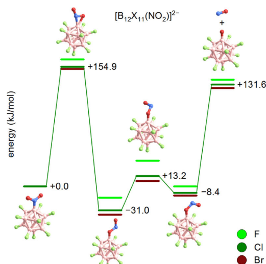
Figure 7. Calculated (B3LYP + GD3BJ/def2-TZVPP) reaction path way for NO • elimination from [B 12 X 11 (NO 2 )] 2− (X = F–Br).
