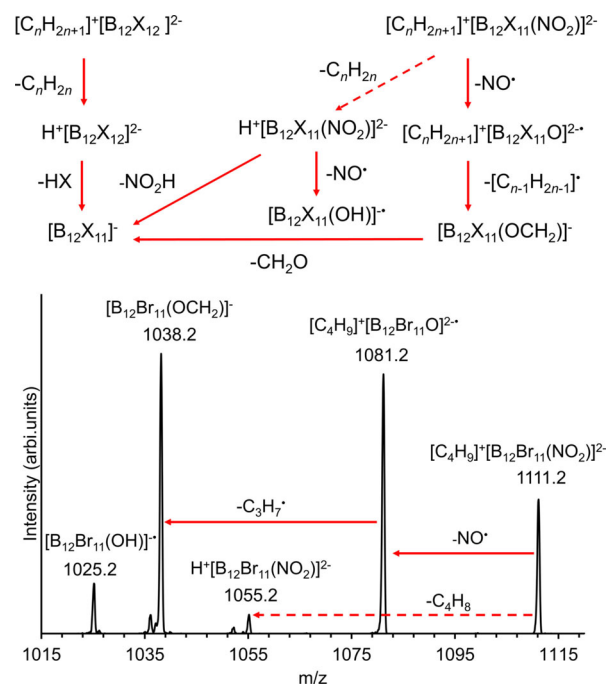
Figure 9. a) Fragmentation scheme of the ion pairs [C_nH_{2n+1}]^+ [B_{12}X_{11}(NO_2)]^{2-} and [C_nH_{2n+1}]^+ [B_{12}X_{12}]^{2-} . While CID of the latter exclusively results in the loss of C_nH_{2n} , this is only a side reaction for [C_nH_{2n+1}]^+ [B_{12}X_{11}(NO_2)]^{2-} (indicated by the dashed arrow) and the loss of the NO is more pronounced. The subsequent loss of [C_{n-1}H_{2n-1}]^* transforms the fragment into the even electron ion [B_{12}X_{11}(OCH_2)]^- . The fragmentation of both ion pairs finally results in [B_{12}X_{11}]^- (for detailed MS^n analysis confirming the shown pathway for X=Br and for exemplary spectra for X=Cl , see section S9 of the Supporting Information). b) CID mass spectrum of the isolated [C_4H_9]^+ [B_{12}Br_{11}(NO_2)]^{2-} ion pair showing the NO and C_3H_7^+ loss as main fragmentation pathways and the C_4H_8 loss as a side reaction (dashed arrow).
