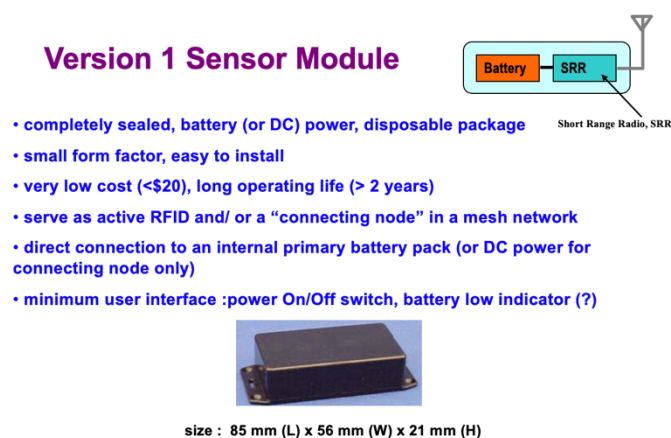
Fig. 11. Version 1 sensor module functions.
