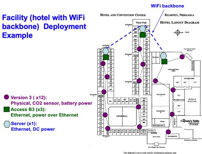
Fig. 29. Proposed deployment of integrated sensor system in a hotel/convention center with Wi-Fi backbone.
