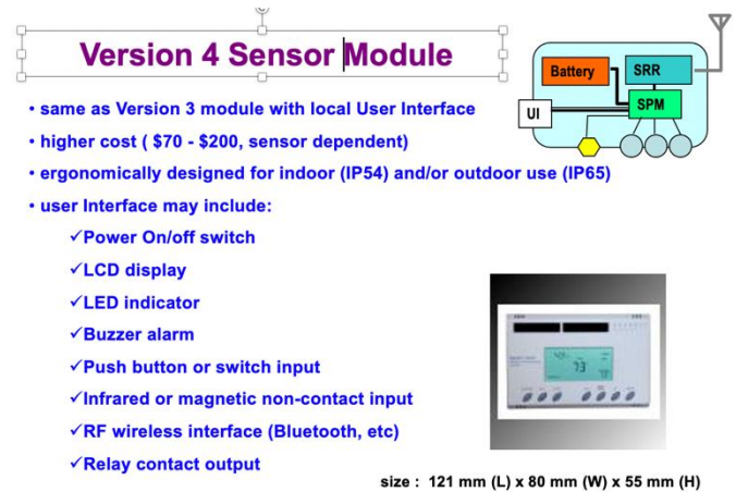
Fig. 17. Version 4 sensor module functions.
