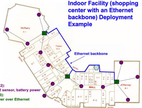
Fig. 28. Proposed deployment of integrated sensor system in an indoor shopping center with wired Ethernet backbone.
