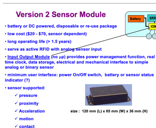
Fig. 13. Version 2 sensor module functions.
