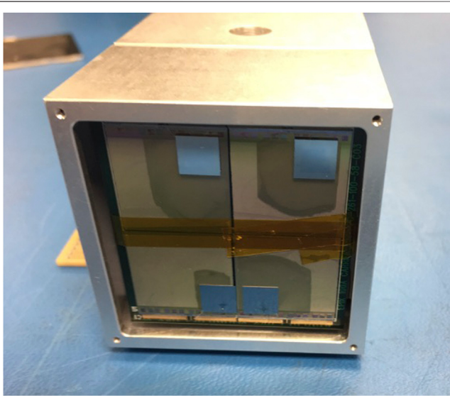
FIGURE 5 | Camera assembled with prototype shallow entrance window sensors bump-bonded to SLAC ePix100 read-out ASIC.
