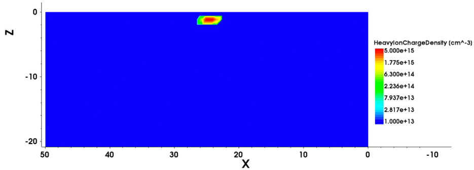
FIGURE 10 | Illustration of photon absorption simulation, showing charge cloud initiated 1 mm (1000 \mu\text{m} ) from the entrance window surface.
