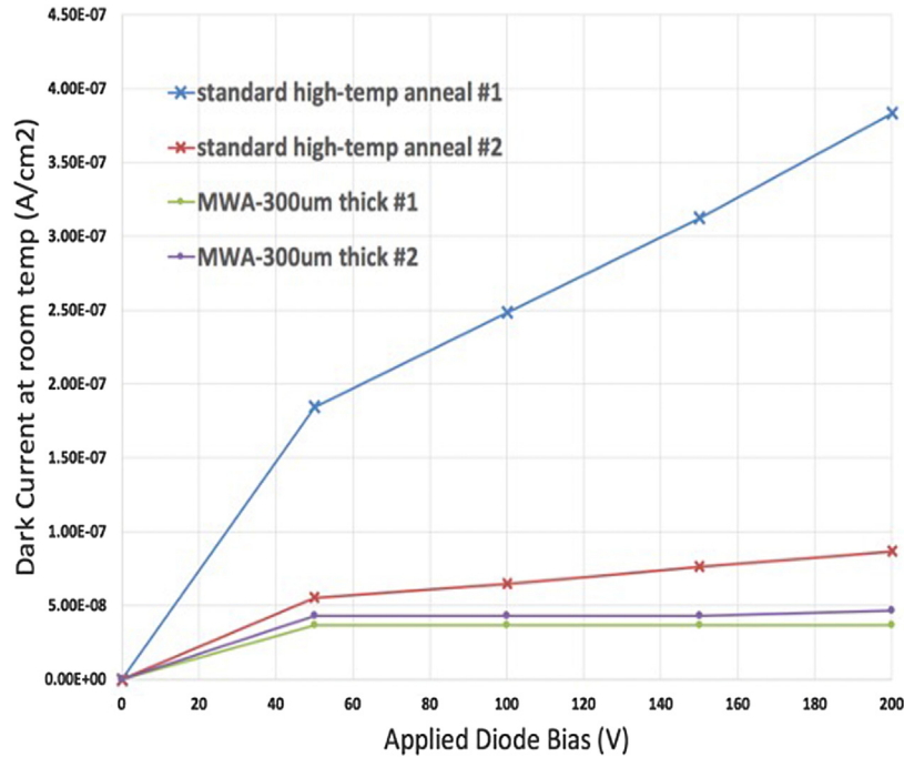
FIGURE 4 | Dark current measured on PIN diodes test structures with conventional anneal and microwave anneal. The microwave annealed sensors have comparable dark current based on this small sample of typical devices.
