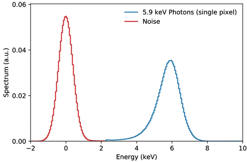
FIGURE 6 | Fe-55 spectrum (shown in blue) measured on planar sensor with microwave annealed entrance window bump-bonded to ePix100 ASIC. Results are comparable to measurements taken with conventional sensors.
