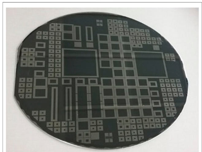
FIGURE 3 | SLAC planar sensor wafer processed at the Stanford Nanofabrication Facility (SNF). The entrance window with patterned metal is shown.
