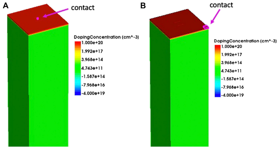
FIGURE 7 | PIN diode structure used for TCAD simulations of x-ray charge collection. (A) (left) has a contact (shown in pink) in the center, where the simulated photon is absorbed. (B) right has an oxide interface over the simulated photon absorption location, with an electrical contact (pink square) in the corner.
