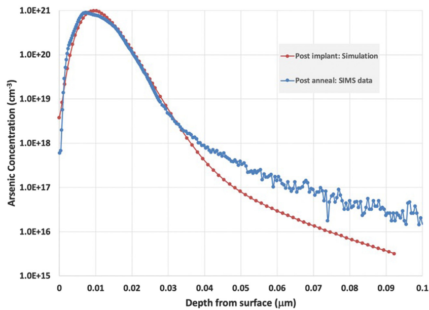
FIGURE 1 | Profile for 10 KeV Arsenic implant: process simulation of post-implanted profile, and experimental results (SIMS data) for the same implant after microwave anneal.
