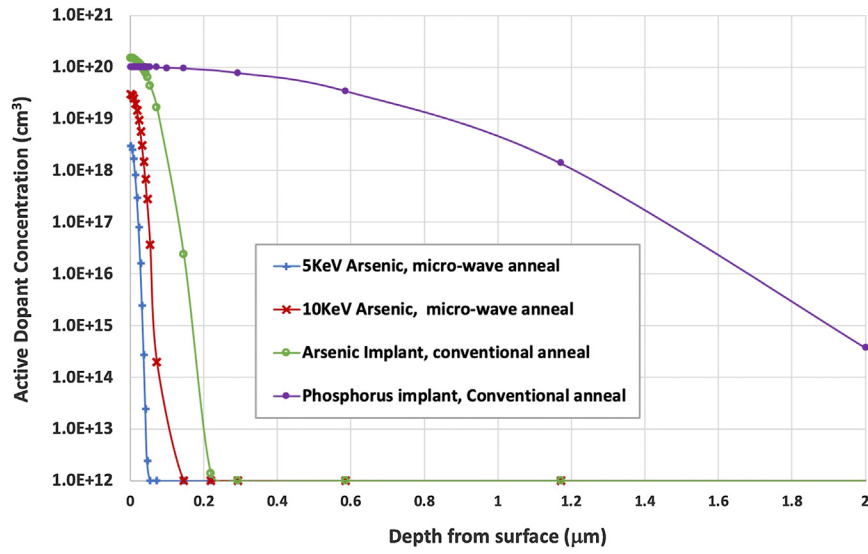
FIGURE 8 | Activated dopant profiles for four entrance window profiles simulated for this work. The spacing of the data points reflects the grid spacing in the vertical direction, which is about 5 nm for the first 50 nm from the surface.
