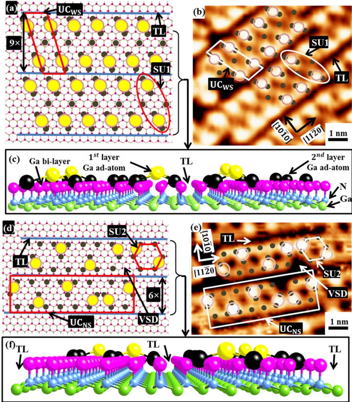
Fig. 5. (Color Online) (a) A top view of the TLS-WS (trench line structure-wide strip) model with SU1 (sub-unit 1) and UC_{ws} (wide strip unit cell), and TL (trench line) indicated; (b) STM image of the TLS-WS with model overlay. Sample bias V_s = -1.5 V, tunnel current I_T = 36.6 pA scanning speed = 120 nm/s; (c) A side perspective view of the TLS-WS (trench line structure-wide strip) model with 1 st layer Ga ad-atom (yellow), 2 nd layer Ga ad-atom (black), Ga ad-layer atom (magenta), N atom (blue), and Ga atom (green); (d) A top view of the TLS-NS (trench line structure-narrow strip) model with SU2 (sub-unit 2) and UC_{NS} (narrow strip unit cell), TL , and VSD (V-shaped defect) indicated; (e) STM image of the TLS-NS with model overlay. Sample bias V_s = -1.85 V, tunnel current I_T = 51.5 pA, scanning speed = 60 nm/s; (f) A side perspective view of the TLS-NS (trench line structure-narrow strip) model with same atomic color key as in (c).
