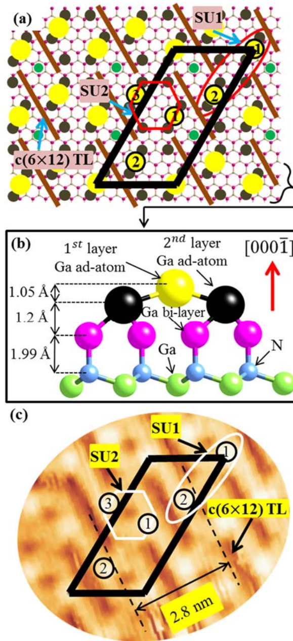
Fig. 4. (Color Online) (a) A top view of the c(6 \times 12) reconstruction model with SU1 (sub-unit 1) and SU2 (sub-unit 2), and c(6 \times 12) TL [ c(6 \times 12) trench line] indicated; (b) A side view of the c(6 \times 12) reconstruction model with 1 st layer Ga ad-atom (yellow), 2 nd layer Ga ad-atoms (black), Ga ad-layer atoms (magenta), N atoms (blue), and Ga atoms (green); vertical spacings based on measurements from Fig. 3; and (c) STM image of the c(6 \times 12) reconstruction. Sample bias V_s = -1.85 V, tunnel current I_T = 51.5 pA, scanning speed = 60 nm/s.
