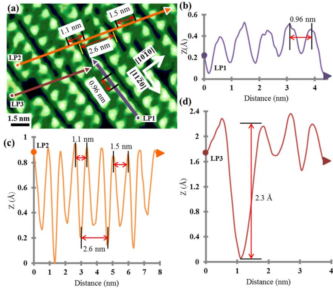
Fig. 3. (Color Online) (a) STM image of the TLS (trench line structure) on GaN (0001̄); (b) showing the line profile LP1, in the [10\bar{1}0] direction; (c) and (d) showing the line profiles LP2 and LP3 in the [11\bar{2}0] direction. Sample bias V_S = -1.5 V, tunnel current I_T = 36.6 pA, scanning speed = 120 nm/s.
