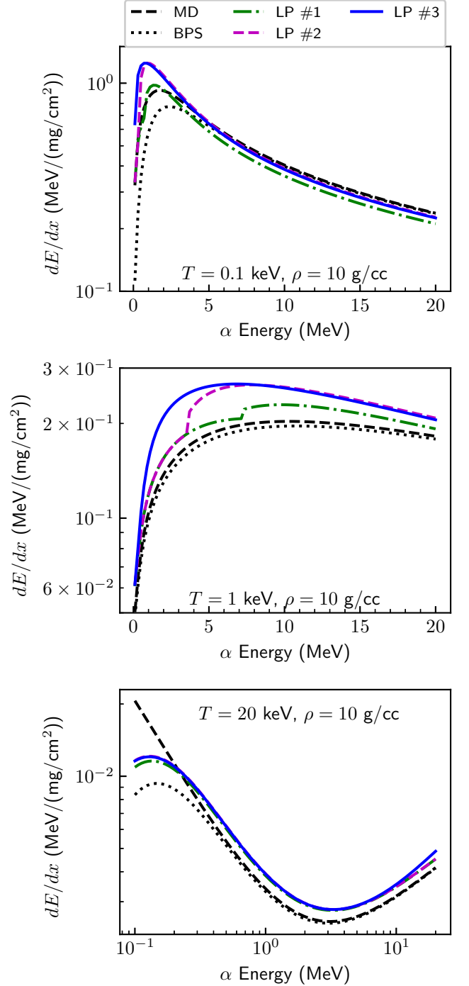
FIG. 1. Three evaluations of the LP stopping power (see text) compared to MD and BPS for \alpha s stopping in a DT plasma at 10 g/cc and 0.1 (top), 1 (center), and 20 keV (bottom).
