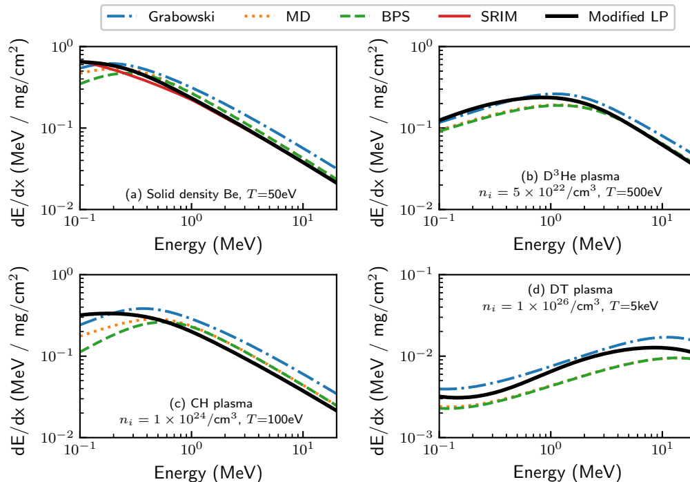
FIG. 2. Comparison of several stopping theories for protons slowing in various ICF-relevant plasmas. (a) Fully-ionized solid-density Be at 50eV (WDM regime), (b) in a D^3He plasma at 500 eV and 5 \times 10^{22}/\text{cm}^3 , (c) in a CH plasma at 10^{24}/\text{cm}^3 and 100eV, relevant to dense shells, and (d) in a high-density and hot DT plasma at 5 keV and 10^{26}/\text{cm}^3 , relevant to ignition targets.
