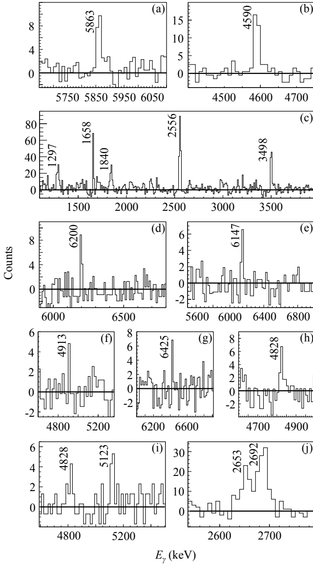
FIG. 7. Random-subtracted \gamma -ray spectra showing all observed transitions from states above 6.0 MeV. All of the spectra were Doppler corrected and gated on tritons populating specific ^{19}\text{Ne} excitation energy ranges. The E_x ranges and other gating parameters are as follows: (a) 5.9–6.7 MeV and the 238-keV \gamma ray, (b) 5.7–6.5 MeV and the 275-keV \gamma ray, (c) 5.8–6.6 MeV and the 238-keV \gamma ray, (d) 6.0–6.8 MeV and the 238-keV \gamma ray, (e) 6.0–6.5 MeV and the 275-keV \gamma ray, (f) 6.0–6.5 MeV and the 1232-keV \gamma ray, (g) 6.2–7.0 MeV and a \gamma -ray multiplicity of 1, (h) 5.7–6.5 MeV and the 275-keV \gamma ray, (i) 6.4–7.0 MeV and the 275-keV \gamma ray, (j) 6.5–7.0 MeV and the 1232-keV \gamma ray.
