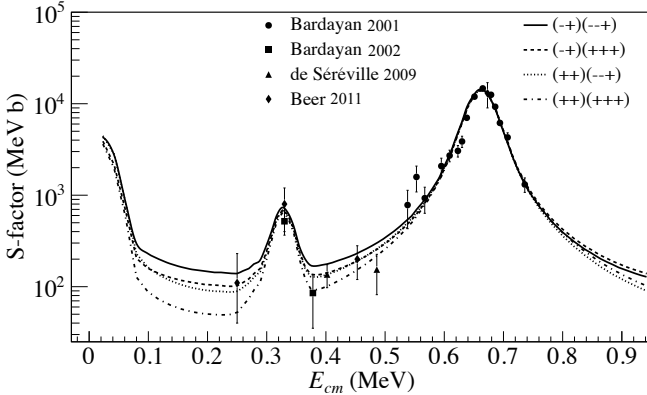
FIG. 8. S-factors calculated for the ^{18}\text{F}(p,\alpha)^{15}\text{O} reaction assuming the combination of interference signs shown. The first (second) set of parentheses shows the interference signs for the 1/2^+ ( 3/2^+ ) states. An energy resolution of 15-keV was included for comparison with experimental data from Bardayan 2001 [11], Bardayan 2002 [31], de Séréville 2009 [35], and Beer 2011 [6]. This figure was adapted from Ref. [9].
