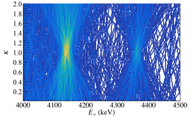
FIG. 3. Gamma-ray spectrum gated on tritons populating excitation energies between 4.0 and 5.0 MeV. The histogram demonstrates how the application of the Doppler correction affects the resolution of the 4140- and 4364-keV \gamma -ray transitions from the 4377- and 4603-keV ^{19}\text{Ne} states, respectively. \kappa is the fraction of \beta_{\text{max}} used, and it is clear that short-lived states require the full correction to be applied to minimize the resolution.
