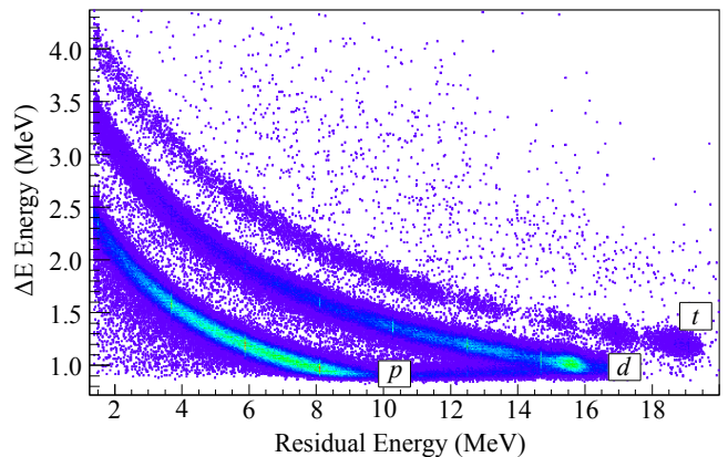
FIG. 1. Particle identification spectrum from the QQQ5 detectors, detected at \theta_{\text{Lab}} = 20^\circ . The elastically scattered ^3\text{He} beam was completely blocked by the aluminum blocker and not detected. Tritons from the reaction of interest are clearly separated from the protons and deuterons produced by the other reactions on the target. Adapted from Ref. [21].
