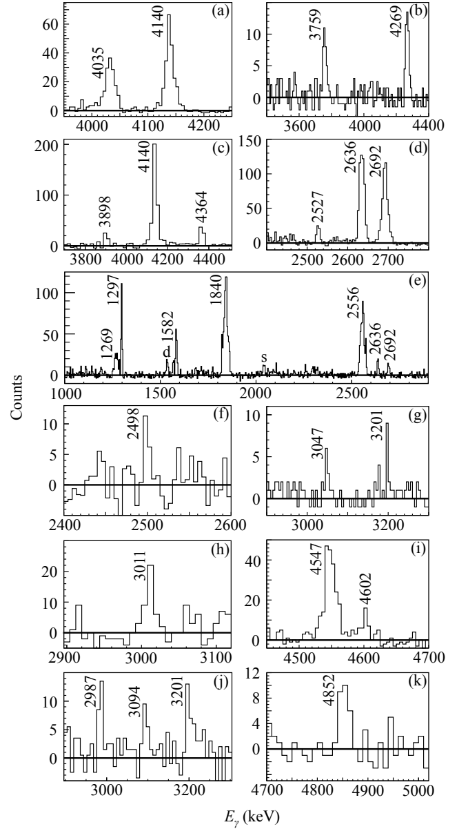
FIG. 6. Random-subtracted \gamma -ray spectra showing all transitions observed from states between 3.0 and 6.0 MeV. All of the spectra were Doppler corrected and gated on tritons populating specific ^{19}\text{Ne} excitation energy ranges. The E_x ranges and other gating parameters are as follows: (a) 3.6 – 4.4 MeV and a \gamma -ray multiplicity of 1, (b) 3.8 – 4.6 MeV and the 275-keV \gamma ray, (c) 3.7 – 4.5 MeV and the 238-keV \gamma ray, (d) 3.7 – 4.5 MeV and the 275-keV \gamma ray, (e) 4.0 – 4.8 MeV and the 238-keV \gamma ray, (f) 3.8 – 4.6 MeV and the 1297-keV \gamma ray, (g) 4.2 – 5.0 MeV and the 1232-keV \gamma ray, (h) 4.4 – 4.9 MeV and the 238-keV \gamma ray, (i) 4.4 – 5.2 MeV and a \gamma -ray multiplicity less than 6, (j) 4.3 – 5.1 MeV and the 275-keV \gamma ray, (k) 4.7 – 5.4 MeV.
