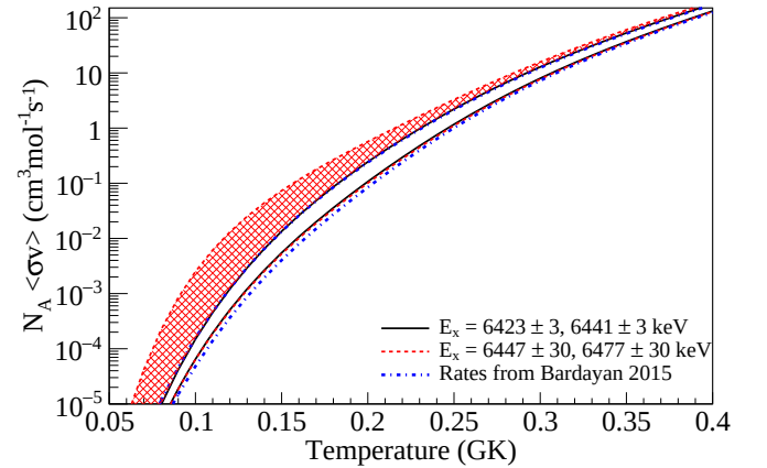
FIG. 9. ^{18}\text{F}(p,\alpha)^{19}\text{Ne} reaction rate calculations showing the reduction in uncertainty from constraining the energies of the 3/2^+ states. The upper limit of the rate is reduced by factors of 1.5-17 in the temperature range of nova nucleosynthesis. The rate calculated by Bardayan 2015 [8] is included for comparison. This figure was adapted from Ref. [9].
