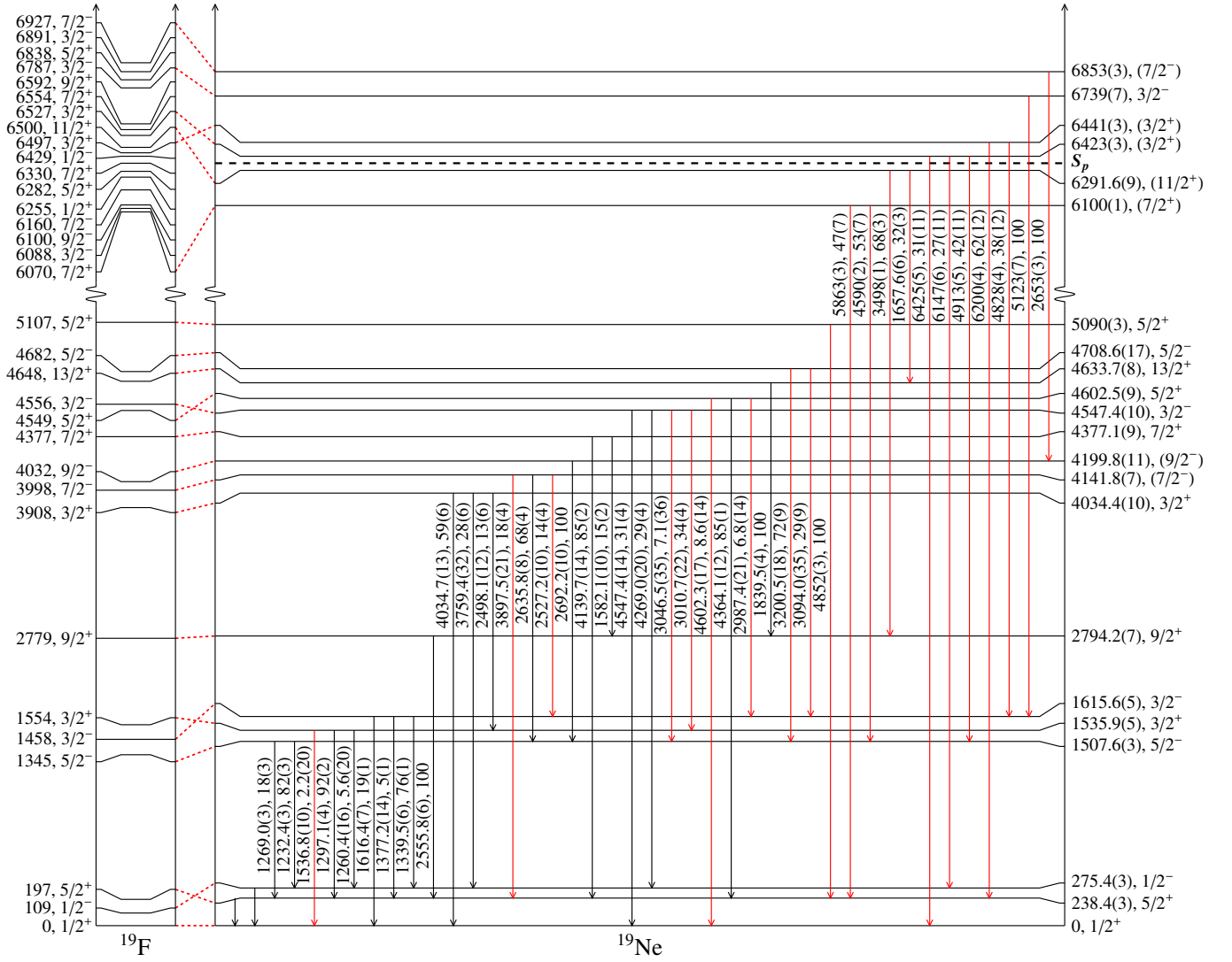
FIG. 4. Level structure of ^{19}\text{Ne} for energy levels (keV) observed in the data, with analog states in ^{19}\text{F} shown to the left with dashed lines. ^{19}\text{F} levels between 5.1 and 6 MeV were omitted for clarity. Transition arrows in black were previously reported. Red arrows signify transitions newly discovered in this work. Gamma-ray energies (keV) and branching ratios (%) are listed next to each transition.
