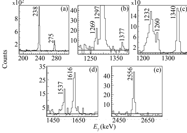
FIG. 5. Random-subtracted low-energy \gamma -ray spectra showing all transitions observed from states with excitation energies less than 3.0 MeV. All of the spectra were Doppler corrected, except for panel (a), and gated on tritons corresponding to specific ^{19}\text{Ne} excitation energy ranges. The E_x ranges and other gating parameters are as follows: (a) 0 – 0.6 MeV, (b) 1.3 – 2.1 MeV and the 238-keV \gamma ray, (c) 1.0 – 1.8 MeV and the 275-keV \gamma ray, (d) 1.0 – 1.8 MeV and a \gamma -ray multiplicity of 1, (e) 2.0 – 2.8 MeV and the 238-keV \gamma ray.
