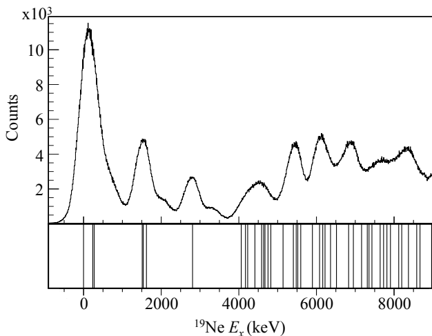
FIG. 2. ^{19}\text{Ne} excitation energy spectrum from one QQQ5 telescope (upper panel) produced by gating on the tritons in Fig. 1. The lower panel shows the locations of previously reported energy levels in ^{19}\text{Ne} , taken from Ref. [22].
