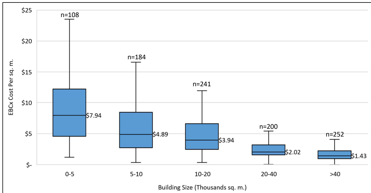
Figure 4. EBCx project cost per square meter ($2017), by building size, with median values indicated (all data)
