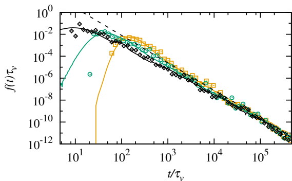
FIG. 2. First passage time distributions at (black) x_1 = 25r_0 , (green) 50r_0 , (orange) 10^2 r_0 from the start plane. Time is rescaled by the advection travel scale \tau_v = r_0/v_0 . Solid lines denote the direct numerical simulations, symbols are the predictions from the stochastic model, the dashed lines shows the t^{-1-\beta} long time scaling with \beta = 3/2 .
