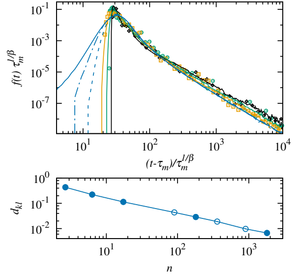
FIG. 5. (top panel) The predicted Lévy stable density (solid blue) and rescaled first passage time PDFs from the (symbols) DFN simulations and (lines) TDRW at distances (black) 25r_0 , (green) 50r_0 and (orange) 10^2 r_0 . The dashed and dash-dotted blue lines show TDRW predictions at distances 10^3 r_0 and 10^4 r_0 from the inlet. The TDRW uses 10^7 particles. (bottom panel) Kullback-Leibler divergence between the rescaled first passage time distributions and the Lévy stable density plotted as a function of number of convolutions. The full circles correspond to the distributions shown in the top panel.
