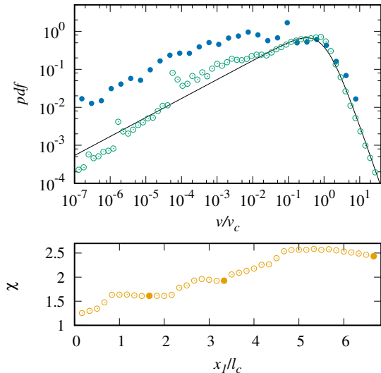
FIG. 4. (top panel) Illustration of (empty circles) steady Lagrangian velocity PDF p_s(v) , (full circles) initial velocity PDF p_0(v) and (solid line) Burr distribution (3). (bottom panel) Tortuosity as a function of streamwise distance. The full circles correspond to the tortuosity values at x_1 = 25, 50, 10^2 r_0 .
