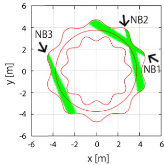
Fig. 4 Fast-ion birth profile produced by NB. Green points represent the birth points projected onto the equatorial plane. Red lines represent the last closed flux surface (LCFS) and the magnetic axis.
