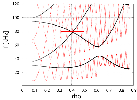
Fig. 8 Alfvén continuous spectra of the toroidal mode numbers n=1 (black) and n=11 (red). The frequency and the spatial location for each AE with frequency f=48, 80, 100 kHz is shown with horizontal line.
