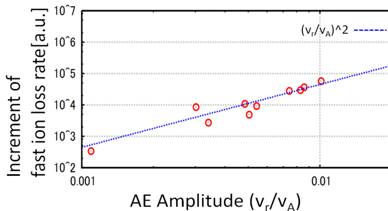
Fig. 10 AE-induced fast-ion loss rate versus maximum AE amplitude (radial MHD velocity normalized by Alfvén velocity) for each burst.
