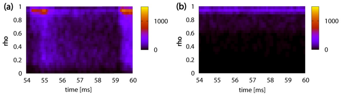
Fig. 16 Time evolution of the initial radial distribution of lost fast-ions produced by co-injected NB for (a) multi-phase and (b) classical simulations. Color represents the number of fast-ions [arb.unit]. The hybrid phase of the multi-phase simulation is 54ms-55ms and 59ms-60ms, and the classical phase where the MHD perturbations are neglected is 55ms-59ms.
