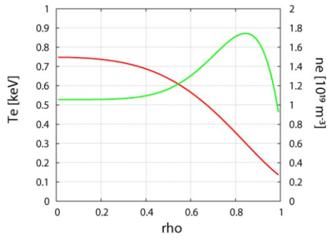
Fig. 3 Electron temperature and density profiles in LHD experiment #90090.
