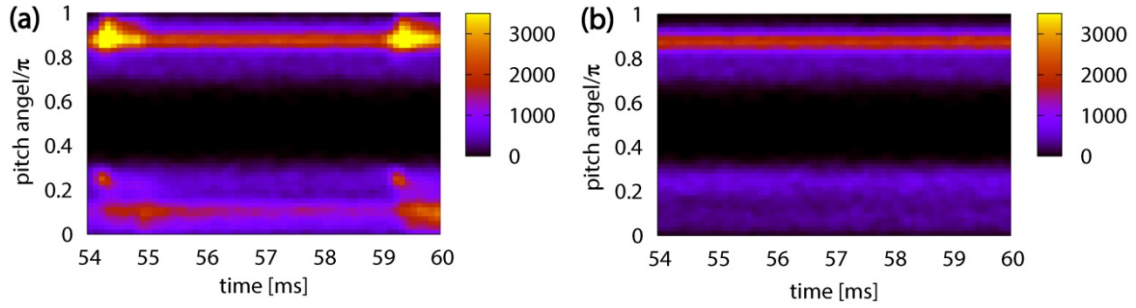
Fig. 15 Time evolution of the initial pitch angle distribution of lost fast-ions for (a) multi-phase and (b) classical simulations. Color represents the number of lost fast-ions [arb.unit]. The hybrid phase of the multi-phase simulation is 54ms-55ms and 59ms-60ms, and the classical phase where the MHD perturbations are neglected is 55ms-59ms.
