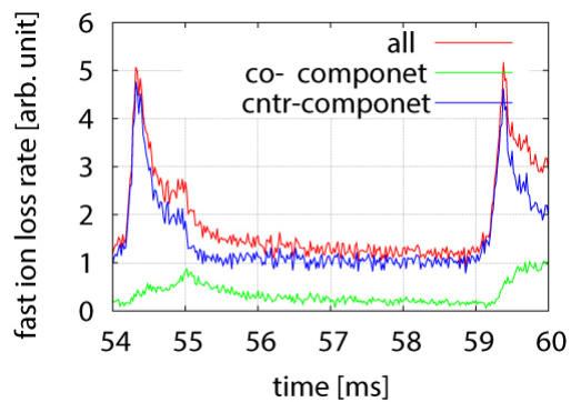
Fig. 11 Time evolution of fast-ion loss rate. Green and blue lines represent the fast-ion loss rate for the fast-ions produced by the co- and the counter-injected NBs, respectively. Red line represents the total fast-ion loss rate. The hybrid phase of the multi-phase simulation is 54ms-55ms and 59ms-60ms, and the classical phase where the MHD perturbations are neglected is 55ms-59ms.
