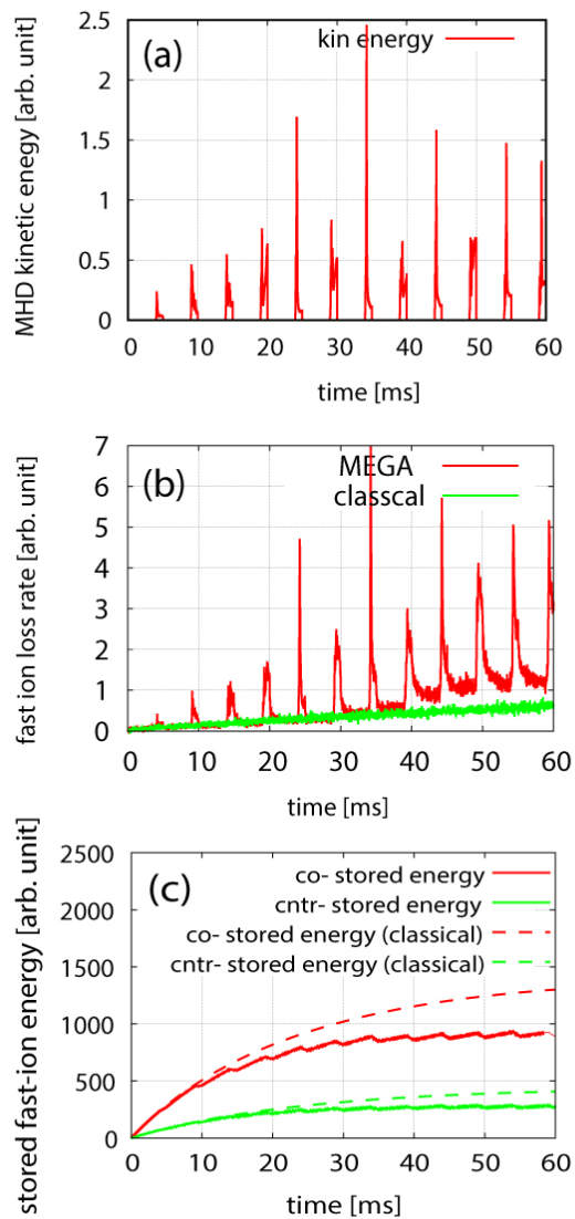
Fig. 5 Time evolutions of (a) MHD kinetic energy of the fast-ion driven instabilities, (b) fast-ion loss rate, and (c) stored fast-ion energy. In panels (b) and (c), the results of the “classical calculation”, which are results of MEGA code without MHD instabilities, are shown together for comparison. In panel (b), fast-ion loss rate does not include the prompt loss particles whose lifetime is less than 50 \mu\text{s} .
