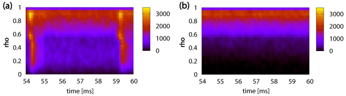
Fig. 17 Time evolution of the initial radial distribution of lost fast-ions produced by counter-injected NB for (a) multi-phase and (b) classical simulations. Color represents the number of fast-ions [arb.unit]. The hybrid phase of the multi-phase simulation is 54ms-55ms and 59ms-60ms, and the classical phase where the MHD perturbations are neglected is 55ms-59ms.
