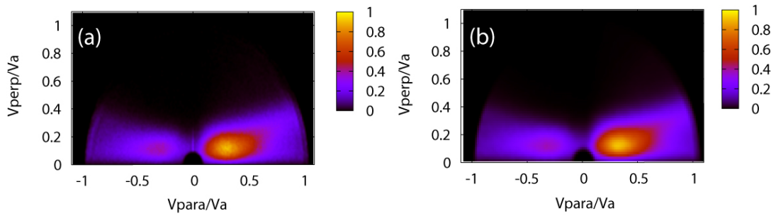
Fig. 1 Fast-ion velocity distribution calculated with (a) MEGA and (b) MORH. Horizontal and vertical axes are parallel and perpendicular fast-ion velocities normalized by the Alfvén velocity, respectively. The color represents the number of fast-ions [arb.unit].
