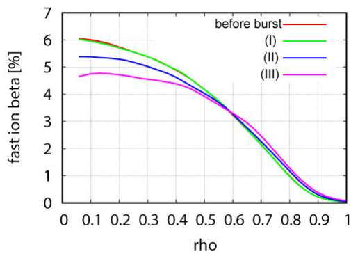
Fig. 9 Fast-ion beta profiles during the burst of the fast-ion driven instabilities. Red, green, blue and purple lines represent the fast-ion beta profiles at 4 moments: (I) the initial peak of MHD
