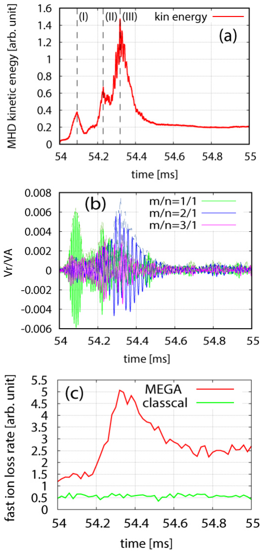
Fig. 6 Time evolutions of (a) MHD kinetic energy, (b) radial MHD velocity harmonics, and (c) fast-ion loss rate during a burst of fast-ion driven instabilities.
