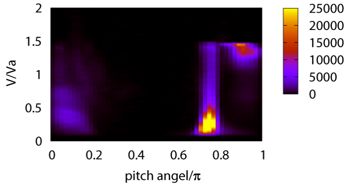
Fig. 14 Velocity space distribution of lost fast-ions. Horizontal axis is pitch angle normalized by \pi , and the vertical axis is the total velocity normalized by Alfvén velocity. Color represents the number of fast-ions [arb. unit].
