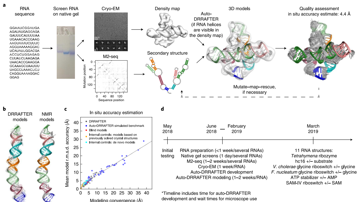
Fig. 1 | The Ribosolve pipeline. RNA structure determination through cryo-EM, M2-seq and computational modeling. a , RNA samples are prepared and screened on a native gel to check for the formation of sharp bands. M2-seq experiments are performed to elucidate the RNA secondary structure. Cryo-EM elucidates the global architecture of the RNA. The M2-seq-based secondary structure and cryo-EM map are used to build all-atom models with auto-DRRAFTER. Model accuracy is predicted from the overall modeling convergence. Helical regions of the 3D models are colored to match the secondary structure diagram. b , Blind HIV-1 DIS DRRAFTER models (left) and NMR models (right). Each helix is depicted with a different bright color. Junctions are colored gray. c , Mean model r.m.s.d. accuracy over the top-ten-scoring models versus modeling convergence for models after each round of auto-DRRAFTER for the benchmark on simulated maps (blue), DIS blind models (red), DRRAFTER models (gray) 11 , and F. nucleatum and V. cholerae glycine riboswitch, Tetrahymena ribozyme, SAM-IV riboswitch, THF riboswitch and B. subtilis T-box-tRNA complex Ribosolve models built into experimental density maps (internal controls, orange and cyan; see Supplementary Table 4). d , Timeline for Ribosolve structure determination in this study.
