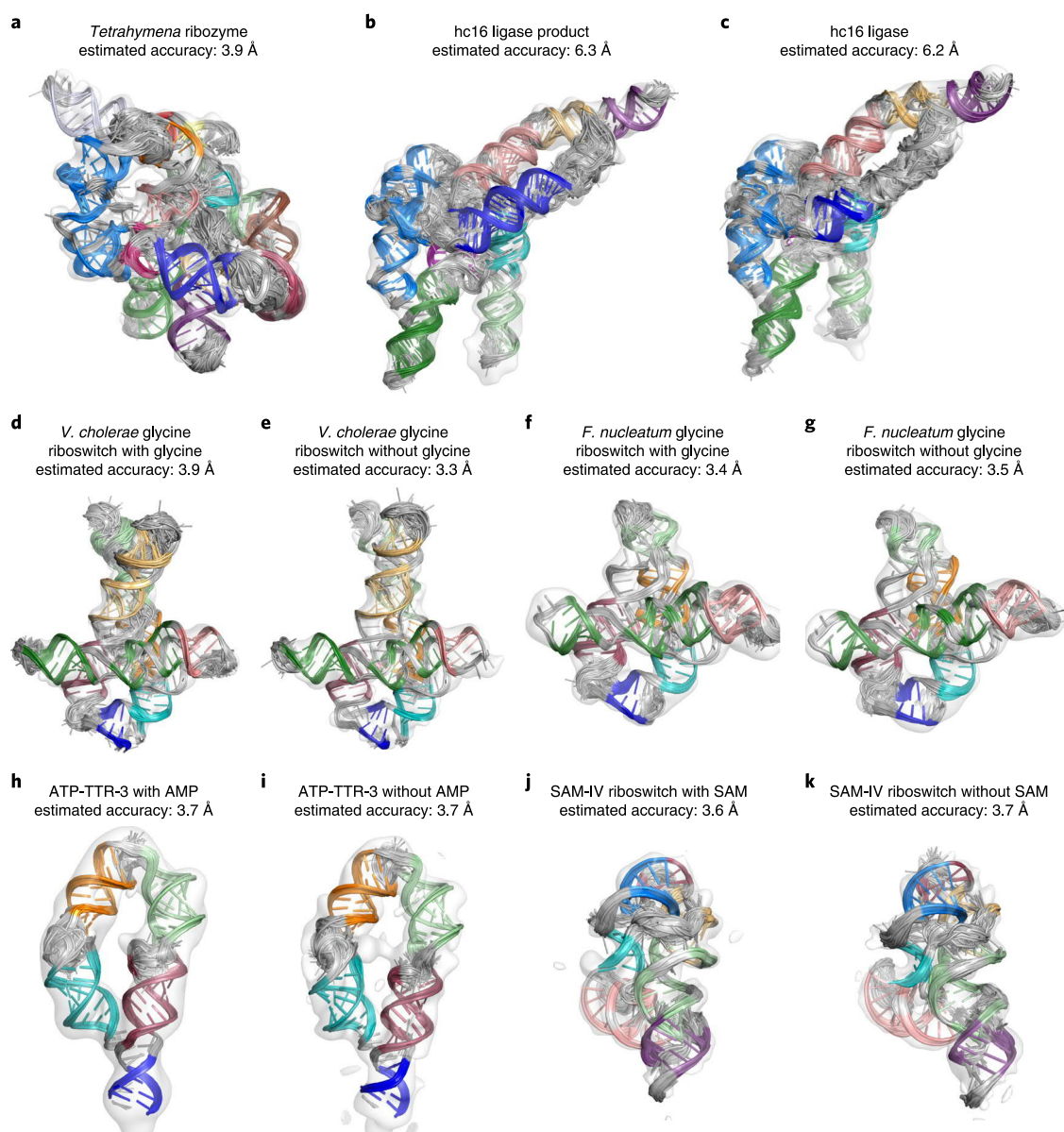
Fig. 3 | RNA structures determined by the Ribosolve pipeline. a–k, Top scoring auto-DRRAFTER models in the cryo-EM maps and estimated accuracies based on modeling convergence for a , Tetrahymena ribozyme, b , hc16 ligase product, c , hc16 ligase, d , V. cholerae glycine riboswitch with glycine, e , V. cholerae glycine riboswitch without glycine, f , F. nucleatum glycine riboswitch with glycine, g , F. nucleatum glycine riboswitch without glycine, h , ATP-TTR-3 with AMP, i , ATP-TTR-3 without AMP, j , SAM-IV riboswitch with SAM, and k , SAM-IV riboswitch without SAM. Each helix is depicted with a different bright color. Nonhelical regions are colored gray.
