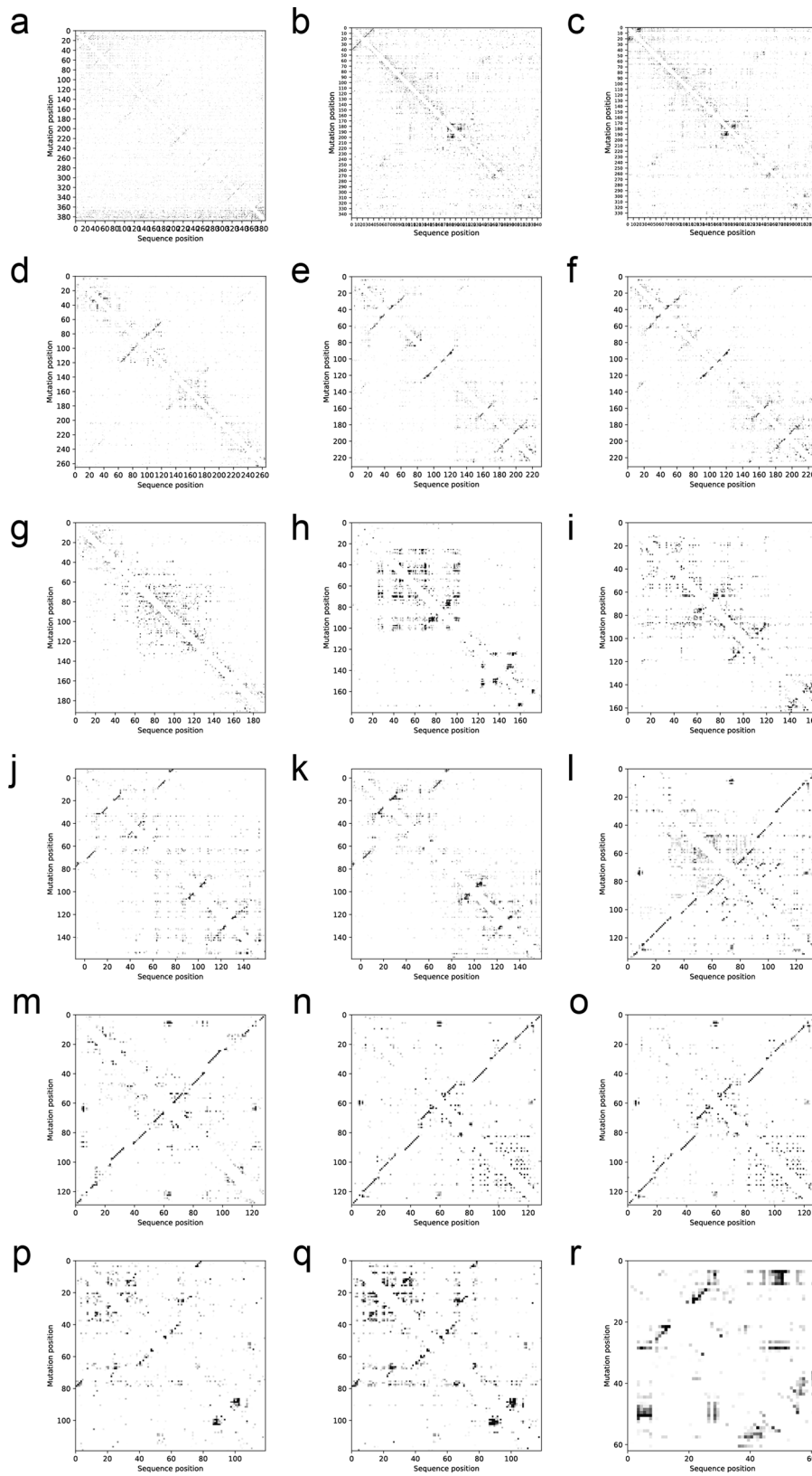
Extended Data Fig. 7 | Experimental M2-seq z-score plots. (a) Tetrahymena ribozyme (n=65041 sequences), (b) hc16 product (n=459852 sequences), (c) hc16 (n=451568 sequences), (d) human scaRNA6 (n=866158 sequences), (e) V. cholerae glycine riboswitch with glycine (n=928767 sequences), (f) V. cholerae glycine riboswitch without glycine (n=974343 sequences), (g) human RB1 5' UTR (n=889700 sequences), (h) 24-3 (n=515486 sequences), (i) human U1 snRNA (n=1185187), (j) F. nucleatum glycine riboswitch with glycine (n=803254 sequences), (k) F. nucleatum glycine riboswitch without glycine (n=670301 sequences), (l) eterna3D-JR_1 (n=994048 sequences), (m) spinach-TTR-3 (n=1090666 sequences), (n) ATP-TTR-3 with AMP (n=914892 sequences), (o) ATP-TTR-3 without AMP (n=712801 sequences), (p) SAM IV riboswitch with SAM (n=131464 sequences), (q) SAM IV riboswitch without SAM (n=991972 sequences), and (r) downstream peptide riboswitch (n=1012081 sequences).
