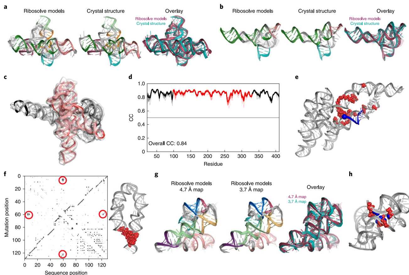
Fig. 4 | Tests of Ribosolve model accuracy. a, b, Top-ten-scoring fully automated Ribosolve models (left; models 2-10 are transparent; each helix depicted with a different bright color; nonhelical regions colored gray), previously solved crystal structures (middle; colors match Ribosolve models) and overlay (right; Ribosolve models colored pink; crystal structure colored cyan) for F. nucleatum glycine riboswitch ( a ) and V. cholerae glycine riboswitch ( b ). Note that auto-DRRAFTER models were built for the complete RNAs, but for clarity only the parts that correspond to the previously solved crystal structures are shown. c, The Tetrahymena ribozyme Ribosolve model in the cryo-EM map. The region derived from a previously solved crystal structure is colored red and regions built de novo are colored black. d, Real-space correlation between the Tetrahymena ribozyme Ribosolve models and cryo-EM map. Colors are the same as in c . Real-space correlation values for each of the top-ten-scoring models built into each half map are shown as thin lines; the average over all top-scoring models is plotted as a thick line ( n=20 independent models). e, The hc16 product Ribosolve model. Invariant and highly variable residues across final sequences from the original in vitro selection 13 shown as red and white spheres, respectively. The site of substrate ligation, the phosphorus atom in residue 1, is shown as a large blue sphere. All other residues are colored gray. f, M2-seq z-score plots (left) with putative tertiary contacts circled in red and Ribosolve models (right) with nucleotides corresponding to the circled regions in the z-score plots shown as red spheres for the ATP-TTR-3 with AMP ( n=914,892 sequences). g, The best-case SAM-IV apo state Ribosolve models built into the 4.7 Å cryo-EM map determined here (left; models 2-10 are transparent; each helix depicted with a different bright color; nonhelical regions colored gray) and a 3.7 Å map 32 (middle; colors match Ribosolve models). Models are shown overlaid on the right (Ribosolve models built into the 4.7 and 3.7 Å maps colored pink and cyan, respectively). h, The fully automated SAM-IV apo state Ribosolve model with nucleotides hypothesized to form the SAM binding pocket shown as red spheres. Homologous nucleotides taken from a previously solved SAM-I riboswitch structure (PDB ID: 2GIS) are overlaid and shown as blue spheres. CC, real-space correlation coefficient.
