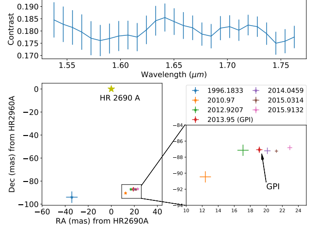
Figure 8. HR 2690 B Recovery. Top: Spectrum (contrast) of the HR 2690 companion measured as the ratio of the secondary to the primary. Bottom: Astrometry of HR 2690 including our GPI epoch. The yellow star marks the position of HR 2690 A.
