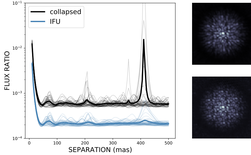
Figure 3. Performance comparison based on internal source data for \lambda -collapsed (black) and IFS data (blue). The contrast is estimated at \text{SNR}=5 . The first half of the data are calibrated with the second half, overestimating performance. The right panel shows snapshots of the data. The IFS provides twice the sensitivity and smooths out low-sensitivity windows at 200 and 400 mas.
