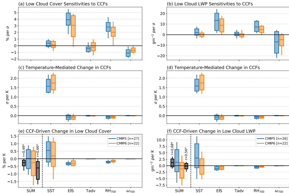
Figure 3. Sensitivities of (a) LCC and (b) LWP_{low} to sea surface temperature ( SST ), estimated inversion strength ( EIS ), surface temperature advection ( Tadv ), relative humidity at 700 hPa ( RH_{700} ), and pressure vertical velocity at 700 hPa ( \omega_{700} ) estimated from climate variability over the SH midlatitude oceans ( 30^\circ - 60^\circ S ) in the piControl simulation. The changes in these factors per unit global warming from the abrupt-4xCO 2 simulation are shown in (c) and (d). Predicted changes in (e) LCC and (f) LWP_{low} due to each cloud controlling factor, estimated as the product of the sensitivities shown in (a) and (b) with the multimodel mean responses of the quantities shown in (c) and (d). Black boxplots show the actual model-produced changes in LCC and LWP_{low} for (left) CMIP5 and (right) CMIP6, above which the across-model correlations between actual and predicted changes are printed. Asterisks indicate statistically significant correlation coefficients ( p < 0.05 ). Boxes extend from the 17th to 83rd percentiles of the model values, with a line at the multimodel average. Whiskers extend to the 5th and 95th percentiles. Anomalies in cloud controlling factors are normalized by the standard deviation of their interannual variations in ERA5 (Copernicus Climate Change Service, 2017) and are therefore expressed in \sigma units, which aids intercomparison of quantities having different units.
