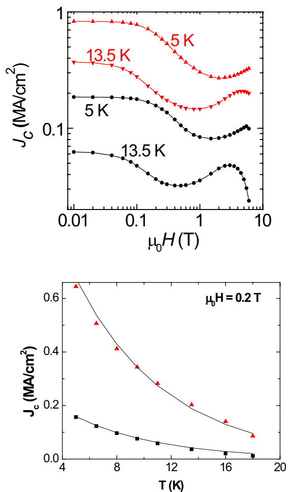
Figure 1. The increase in superconducting critical current density ( J_c ) for annealed optimally-doped \text{Ba}(\text{Fe}_{1-x}\text{Co}_x)_2\text{As}_2 crystal. For x = 0.063 and as-grown (in black) and annealed (in red) crystals, (a) field dependence of critical current density ( J_c ) below T_c , and (b) temperature dependence of J_c at 0.2 Tesla.
