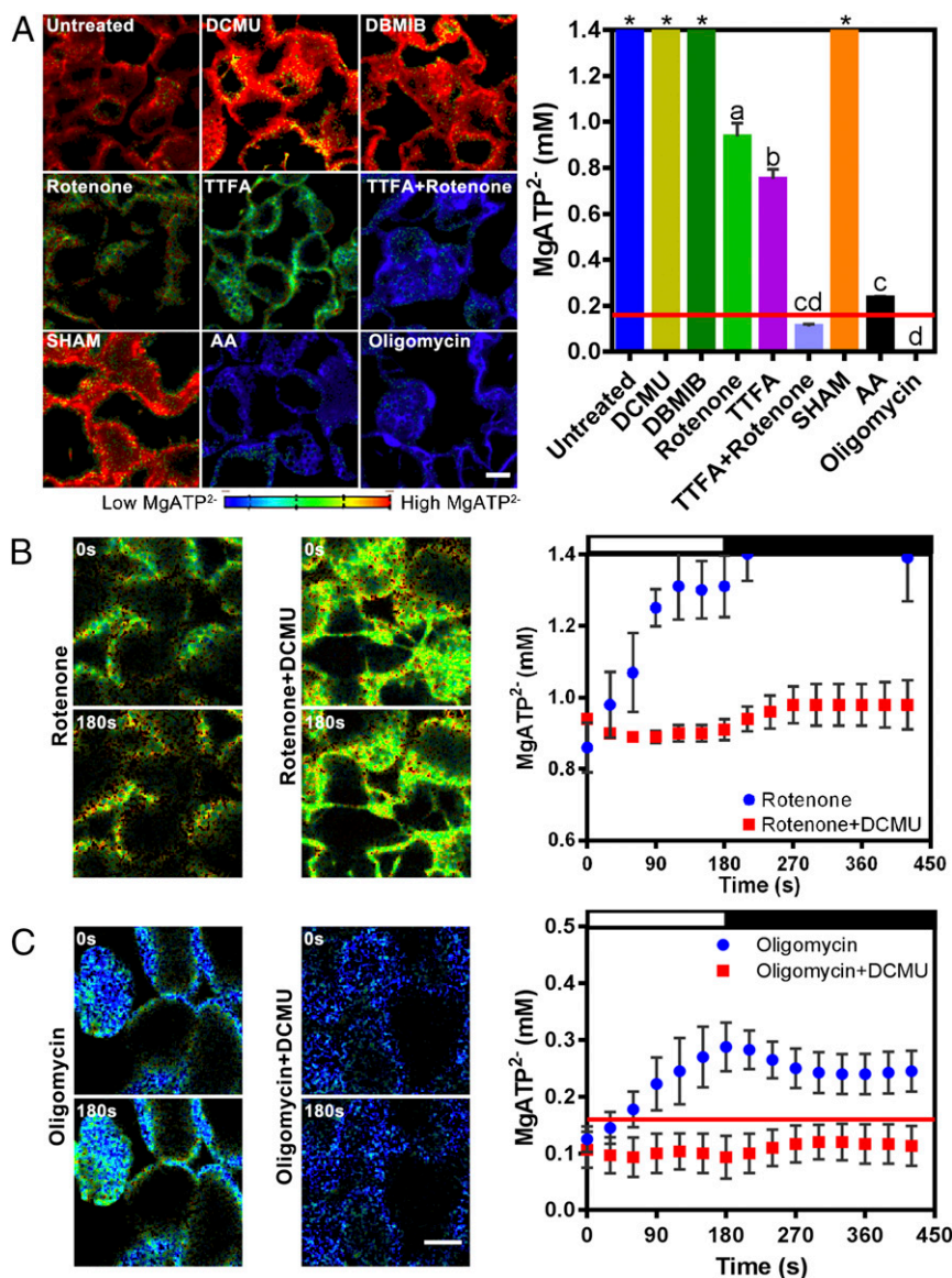
Fig. 4. Contribution of mitochondrion to cytosolic MgATP 2- concentration. (A) Apparent cytosolic MgATP 2- concentrations in cotyledon cells of 10-d-old Arabidopsis seedlings in darkness assessed by stably expressed AT1.03-nD/nA. The means ( \pm SEM) of eight plants are shown in the bar chart. Groups with significant difference by one-way ANOVA with post hoc Tukey HSD test ( P < 0.05 ) are indicated by different letters. The groups marked by asterisks are significantly different from the groups marked by letters, but whether they have intergroup differences is not known. [Scale bar (all panels): 20 \mu m.] The red line indicates the lower detection limit of AT1.03-nD/nA (0.16 mM). (B and C) The change of cytosolic MgATP 2- concentration in illuminated (296 \mu mol·m -2 ·s -1 ) cotyledon ( n = 3 ; mean \pm SEM). The black and white bars indicate dark and illumination period, respectively. [Scale bar (all panels): 20 \mu m.] The red line indicates the lower detection limit of AT1.03-nD/nA (0.16 mM).
