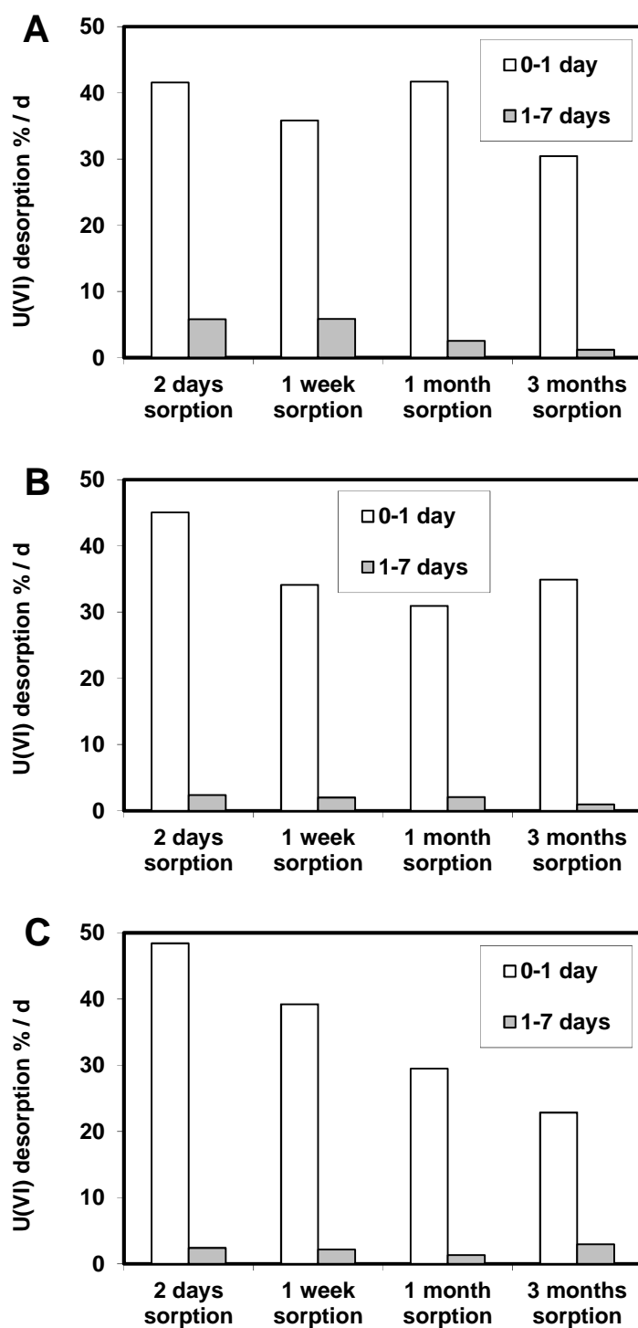
Fig. 5. U(VI) desorption rate in % per day (first 1 day and day 1 to day 7) during the 1-week desorption by 10 mM NaHCO 3 solution after sorption of 50 μM U(VI) to the low Fe soil (A), the medium Fe soil (B), and the high Fe soil (C) over 2 days, 1 week, 1 month, and 3 months in the presence of 2.5 mM Ca 2+ and 5 mM HCO 3 - .
