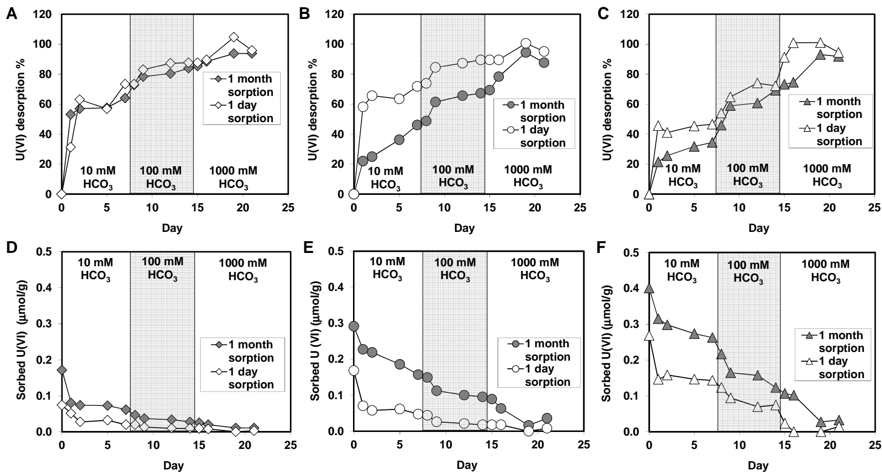
Fig. 9. Sequential desorption kinetics of U(VI) by 10, 100, and 1000 mM NaHCO 3 solutions for a total of 3 weeks (1 week for each desorption step) after sorption of 50 μM U(VI) to saprolite soils (Low Fe: A and D, Medium Fe: B and E, High Fe: C and F) in 0.1 M NaNO 3 solutions containing 2.5 mM Ca 2+ and 5 mM HCO 3 - for 1 day and 1 month.
