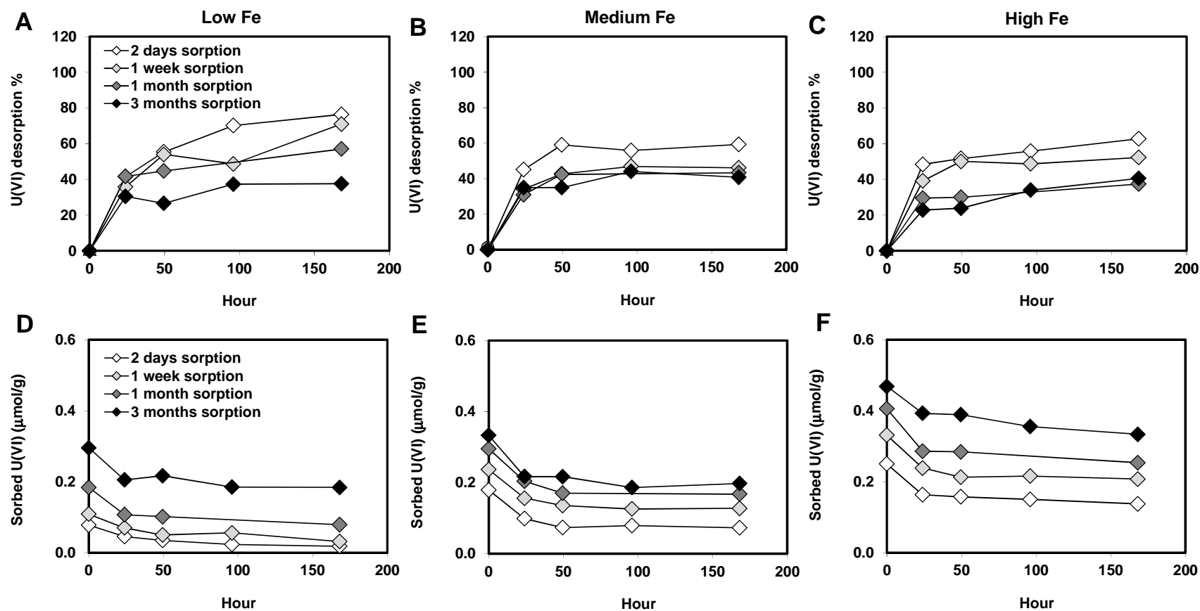
Fig. 4. Percentage of U(VI) desorption and the amount of U(VI) sorbed to saprolite soils (A and D: low Fe, B and E: medium Fe and C and F: high Fe) during the 1-week desorption by 10 mM \text{NaHCO}_3 solution after sorption of 50 \mu\text{M} U(VI) in the presence of 2.5 mM \text{Ca}^{2+} and 5 mM \text{HCO}_3^- over 2 days, 1 week, 1 month, and 3 months.
