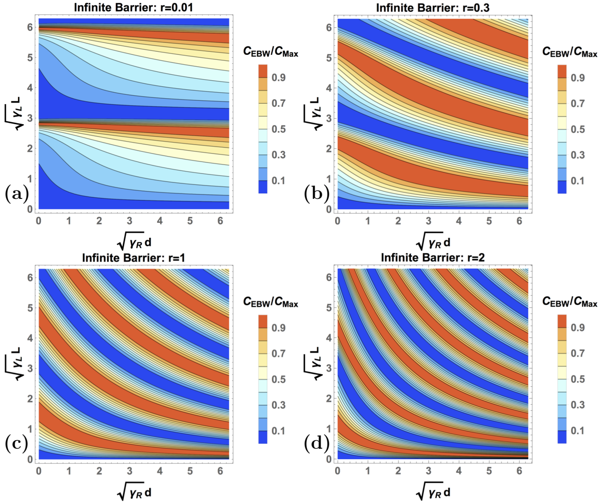
Figure 4. Contour plots showing the variation of the oscillatory factor \cos^2(\phi_{IB}) for the Infinite Barrier model of the X-B mode-conversion efficiency as the distance between the right-hand cutoff and the upper hybrid resonance ( d ), and the distance between the upper hybrid resonance and the left-hand cutoff ( L ) are varied. When L and d are specified, the Infinite Barrier model remains underdetermined via the additional asymmetry parameter r . In all plots, r is constrained to take selected constant values.
