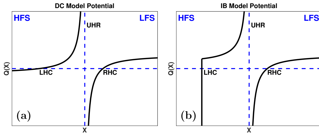
Figure 1. Two choices of model potential function Q(x) for the X-B mode-conversion in 1-D. (a) ‘Double-cutoff’ model, which generates the cutoff-resonance-cutoff triplet with two Budden potentials. (b) ‘Infinite Barrier’ model, which generates the cutoff-resonance-cutoff triplet with a Budden potential and an infinite barrier.
