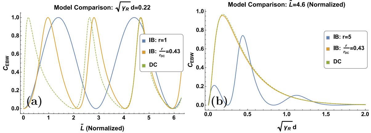
Figure 6. Variation in the X-B mode-conversion efficiency for the Infinite Barrier and the Double-cutoff X-B phase models at (a) fixed d and varying L , and at (b) fixed L and varying d . In these plots, the free parameter r of the IB model is constrained either to take a selected constant value, or to vary analogously with the DC model constraint. We use the notation \tilde{L} to denote generically that L is normalized according to the prescriptions used in figures 3 and 4, that is, \tilde{L} = \sqrt{\kappa_L} L for the DC model, and \tilde{L} = \sqrt{\gamma_L} L for the IB model.
