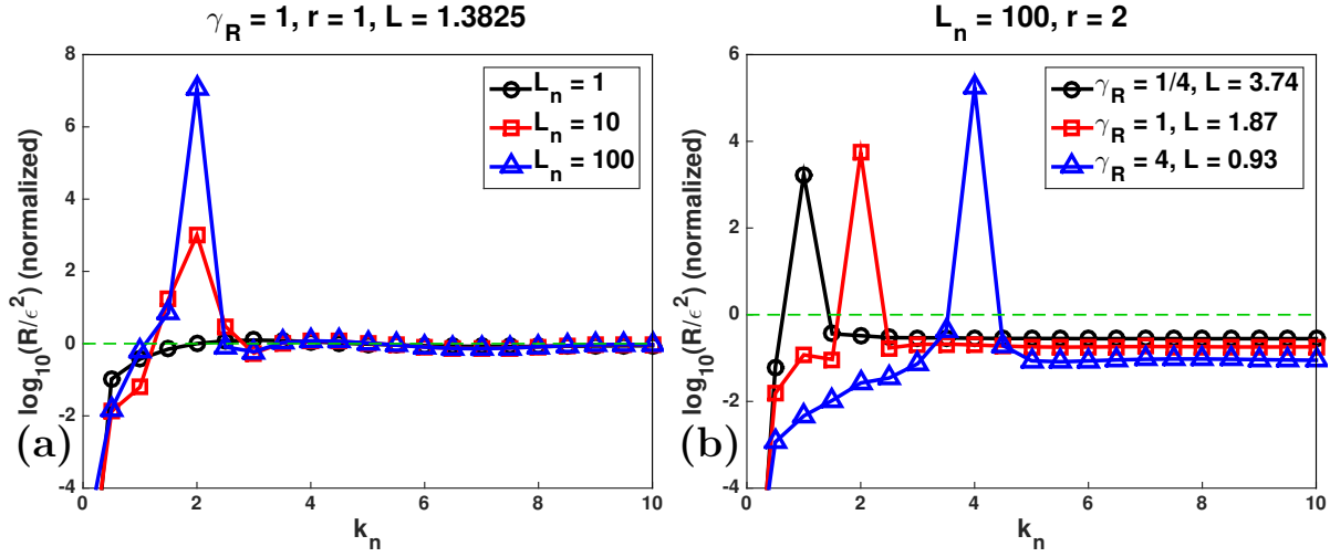
Figure 8. The modified reflection coefficient normalized by the squared fluctuation amplitude \epsilon^2 . (a) Variation in R/\epsilon^2 as the fluctuation wavenumber k_n and the fluctuation decay length L_n are varied, while the launched X-mode wavenumber \sqrt{\gamma_R} is held constant, with no asymmetry ( r = 1 ) in the equilibrium. (b) Variation in R/\epsilon^2 as the fluctuation wavenumber k_n and the launched X-mode wavenumber \sqrt{\gamma_R} are varied, while the fluctuation decay length L_n is held constant, with small asymmetry in the equilibrium. In both figures, all traces are presented on a log-scale, and normalized by their asymptotic values computed with equations 43a and 43b; for (a) this value is \sim 0.71 \cdot L_n^{-2} , while for (b) these values are 5.89 , 0.15 , and 4.72 \times 10^{-3} , for \gamma_R = 1/4 , \gamma_R = 1 , and \gamma_R = 4 respectively. In all cases, the parameters are chosen such that if the density fluctuations were absent ( \epsilon = 0 ), the X-B mode-conversion efficiency would be 100% ( R = 0 ).
