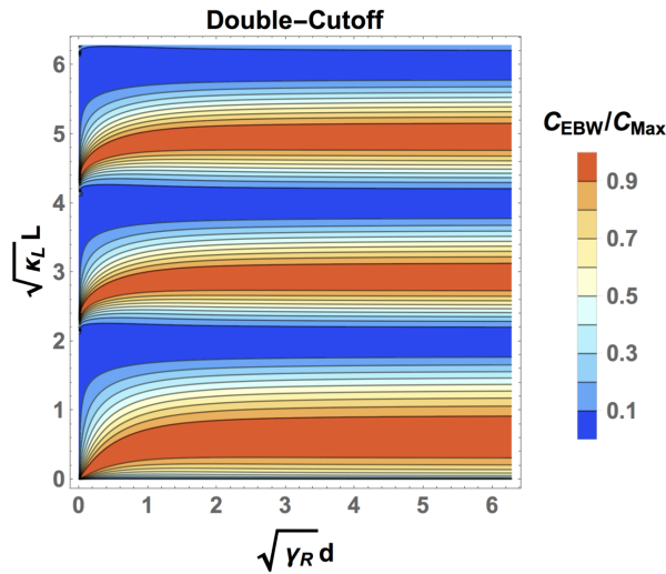
Figure 3. Contour plot showing the variation of the oscillatory factor \cos^2(\phi_{\text{DC}}) for the Double-cutoff model of the X-B mode-conversion efficiency as the distance between the right-hand cutoff and the upper hybrid resonance ( d ), and the distance between the upper hybrid resonance and the left-hand cutoff ( L ) are varied. When L and d are specified, the Double-cutoff model is completely determined.
