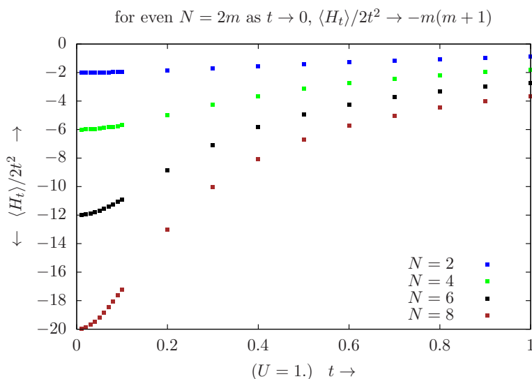
Figure 10. Hopping VEV for even N = 2m case.
