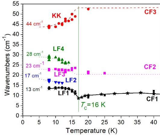
FIG. 3 (color online) Energies of the LF, KK, and CF modes vs temperature. Experimental data for energies of the LF, KK, and CF modes are shown with solid symbols. Data from [39] obtained with conventional linearly-polarized light are shown with dashed curves for comparison. Solid black curve guides the eye.
