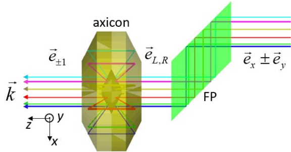
FIG. 1 (color online) Linearly polarizer THz radiation is converted into vortex beam modes \vec{e}_{\pm 1} using a combination of a Fresnel prism (FP) and axicon. After passing through a two-bounce FP retarder, the linearly polarized light \vec{e}_x \pm \vec{e}_y becomes circularly polarized \vec{e}_{L,R} . After passing through the axicon, the beam acquires a vortex phase \vec{e}_{\pm 1} , while losing its circular polarization.
