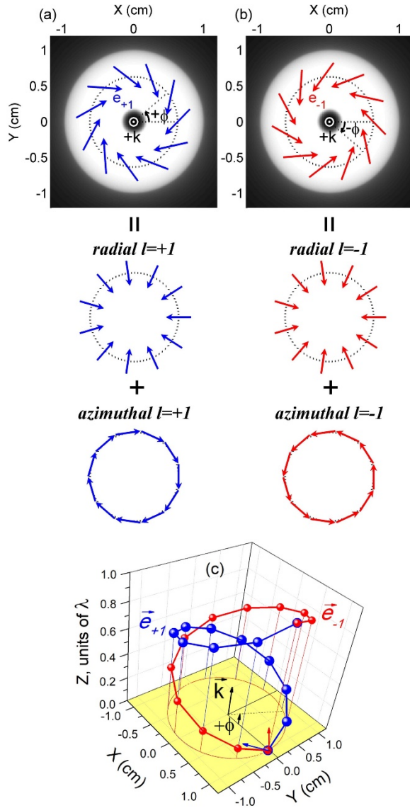
FIG. 2 (color online) Calculated radially-independent electric fields and equal phase trajectories in the vortex beams. (a,b) Projections of electric field for the \vec{e}_{+1} and \vec{e}_{-1} modes are shown in the x - y plane. The white areas represent the intensity distribution of the vortex beam. The beam propagation direction \vec{k} is along the positive z -axis. Decoupling of the vortex modes into the azimuthal and radial ones is also shown. (c) Spatial variation of the equal phase trajectories. \vec{e}_{+1} and \vec{e}_{-1} form the right-hand and left-hand spirals. The corresponding electric field vectors in the x - y plane at z=0 and \phi=0 are shown with red and blue arrows.
