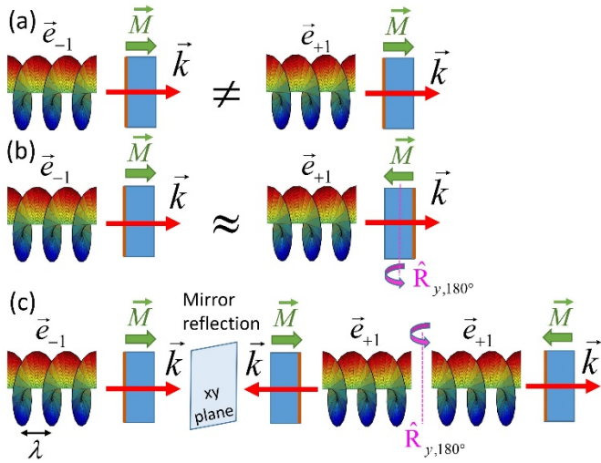
FIG. 5 (color online) Schematics of the observed dichroic effects. Propagation of the wave-front in the vortex beam is illustrated with color rendering. The closest distance between the same colors along the z -direction corresponds to the wavelength of light \lambda . (a) Vortex beam dichroism: \{\vec{k}, \vec{e}_{-1}, \vec{M}\} \neq \{\vec{k}, \vec{e}_{+1}, \vec{M}\} . (b) Same for the observed inversion of the selection rules for rotation of the magnetized sample that also resulted in the sign change for \rho_{\pm 1} . (c) Transformation between \{\vec{k}, \vec{e}_{-1}, \vec{M}\} and \{\vec{k}, \vec{e}_{+1}, -\vec{M}\} can be obtained by applying a mirror reflection that is perpendicular to z and rotation around the y -axis, both for the whole experimental setup. The sample is shown with blue rectangles with green arrows for the sample magnetization direction \vec{M} . One of the sample faces is marked with the vertical brown line.
