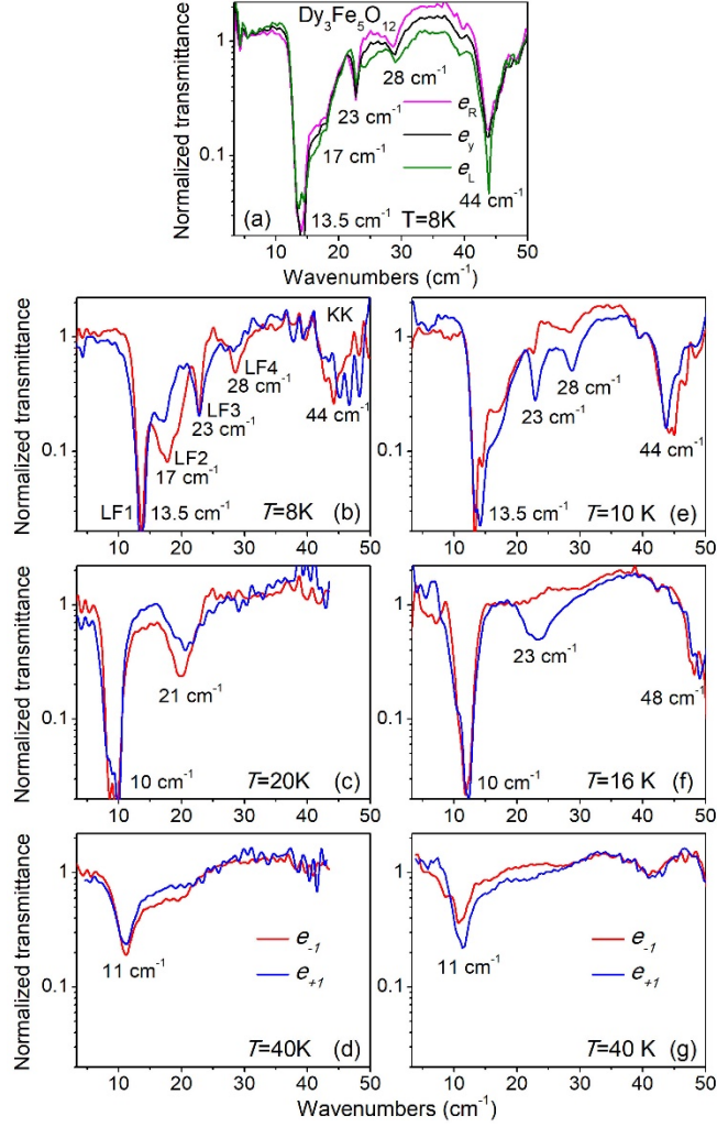
FIG. 4 (color online) Magnetic dichroism in transmittance spectra for circularly polarized light and vortex beams. (a) Normalized transmittance spectra for circularly polarized light \vec{e}_R and \vec{e}_L , and for conventional linearly polarized light \vec{e}_y . The magnetization vector \vec{M} is antiparallel to \vec{k} . (b,c,d) Normalized transmittance spectra for three temperatures and two orthogonal vortex beams \vec{e}_{+1} (blue spectra) and \vec{e}_{-1} (red spectra) measured for \{\vec{k}, \vec{e}_{\pm 1}, \vec{M}\} with the magnetization vector \vec{M} parallel to \vec{k} . (e,f,g) The same for the opposite directions of the light propagation with respect to the sample: \{\vec{k}, \vec{e}_{\pm 1}, \hat{R}_{y,180^\circ}(\vec{M})\} with the magnetization vector \vec{M} antiparallel to \vec{k} . All experimental data in (a-g) are normalized to that measured at T=75 K.
