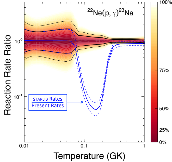
FIG. 19: (color online) The ratio of the STARLIB ^{22}\text{Ne}(p,\gamma)^{23}\text{Na} reaction rate to the present rate is shown in blue with dashed blue lines representing 1- \sigma uncertainties. The present rate is shown centered on the ratio = 1 line in varying shades of red-yellow indicating varying levels of uncertainty in the reaction rate at each temperature.
