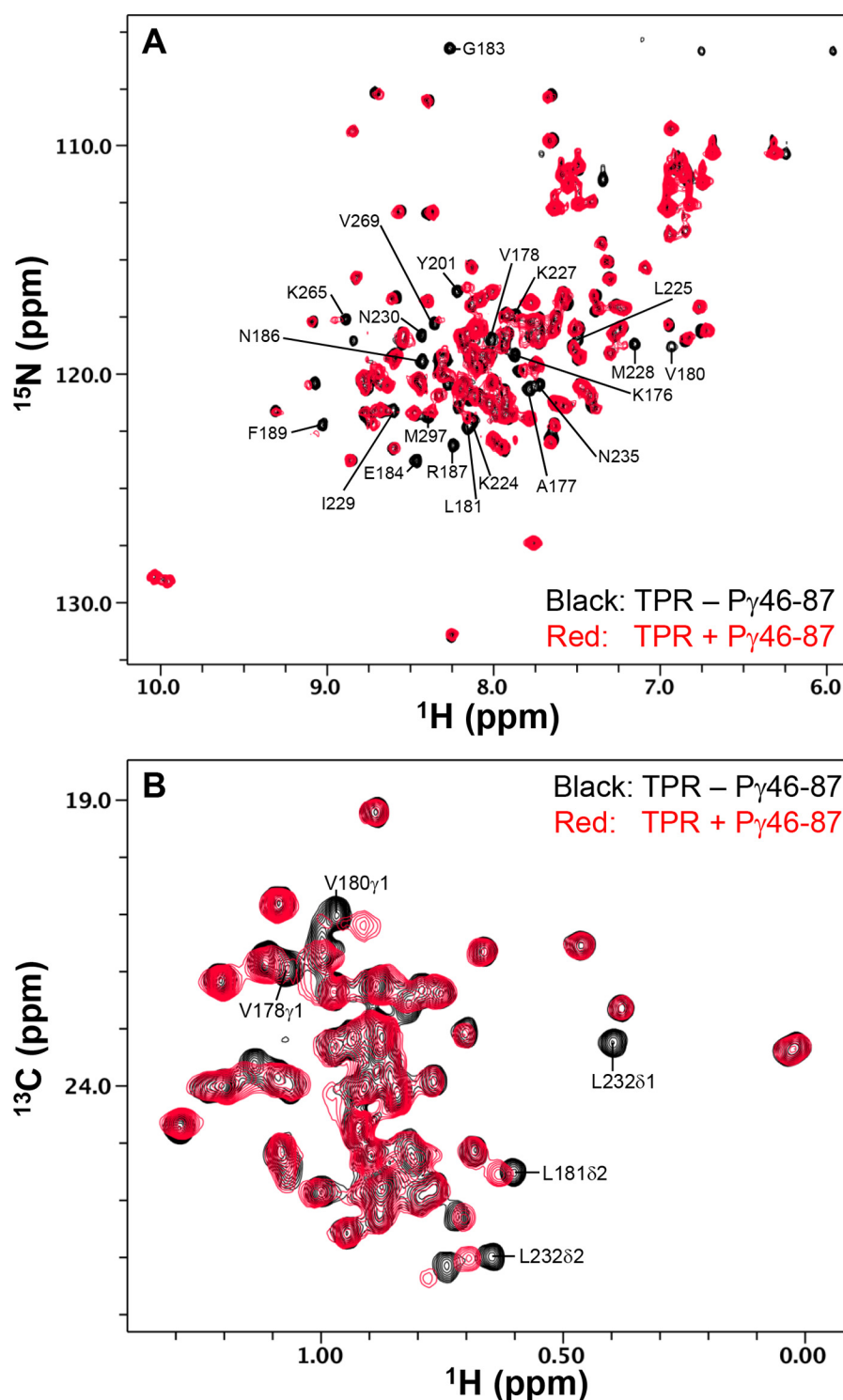
Figure 1. NMR spectra of human uniformly ^{15}\text{N} - and ^{13}\text{C} -methyl (IVL)-labeled AIPL1 TPR domain acquired in the presence and absence of P \gamma 46–87. A, overlay of ^{15}\text{N}/^1\text{H} HSQC spectra. B, overlay of ^{13}\text{C}/^1\text{H} HSQC spectra. The significantly perturbed backbone amide and methyl peaks upon P \gamma peptide binding are labeled using the WT protein sequence numbering. In these experiments, the TPR and P \gamma peptide concentrations used were 157 and 166 \mu\text{M} , respectively.
