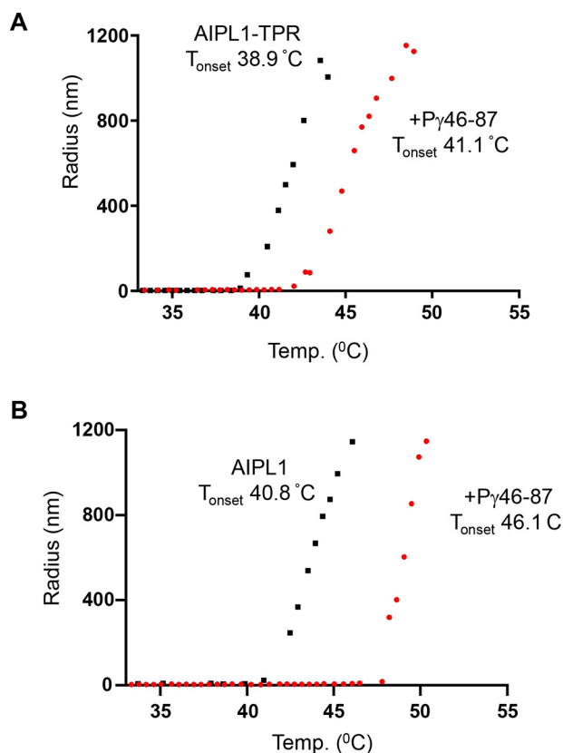
Figure 2. Thermal denaturation, as determined by DLS, for 165 \mu\text{M} AIPL1-TPR (A) and for 135 \mu\text{M} AIPL1(1-316) (B) in the absence (squares) or presence of 330 \mu\text{M} of P \gamma 46-87 (circles). Representative experiments are shown. For experiments performed in triplicate, T_{m-onset} (°C) values are: AIPL1-TPR, 39.0 \pm 0.4 ; AIPL1-TPR + P \gamma 46-87, 41.7 \pm 0.3 ; AIPL1(1-316), 41.0 \pm 0.3 ; and AIPL1(1-316) + P \gamma 46-87, 45.4 \pm 0.2 (means \pm S.E.). Temp., temperature.
