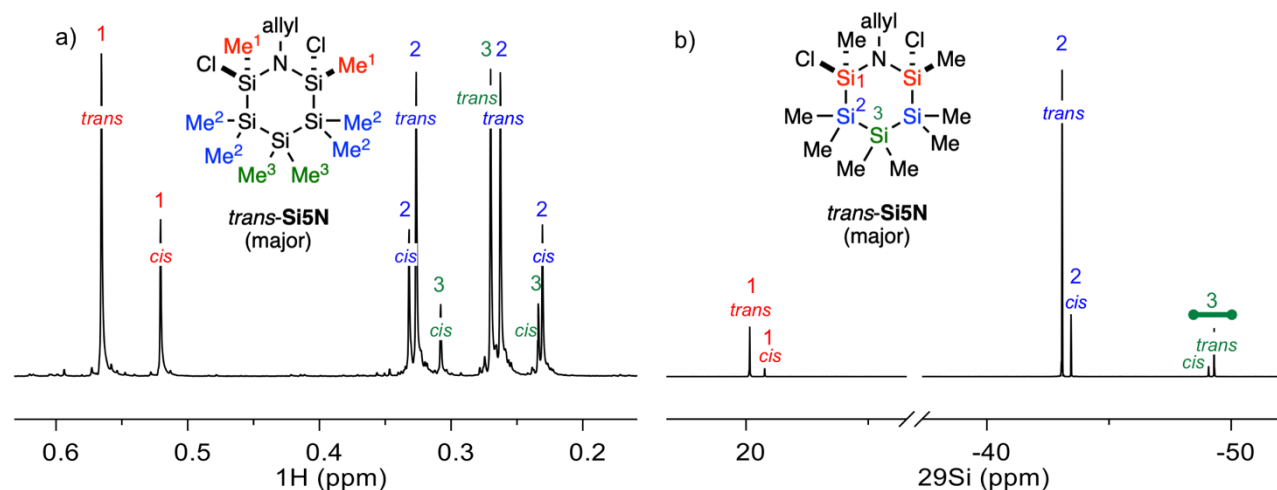
Figure 2. a) Cropped ^1\text{H} NMR spectrum (400 MHz, \text{CDCl}_3 ) highlighting methyl region. b) Cropped ^{29}\text{Si} \{^1\text{H}\} DEPT NMR spectrum (79 MHz, \text{CDCl}_3 ). Assignments based on ^1\text{H} - ^{29}\text{Si} HMBC spectrum (Figure S1).
