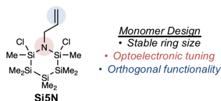
Figure 1. Design of Si5N monomer.
