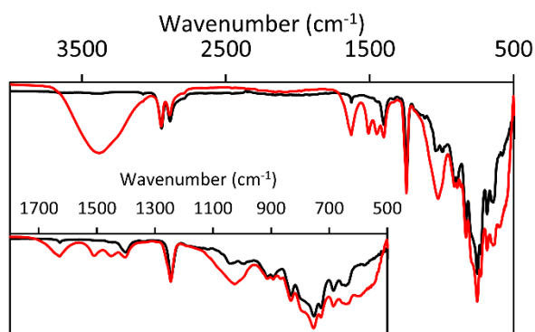
Figure 4. Attenuated Total Reflectance-Fourier Transform Infrared Spectra (ATR-FTIR) of P2 (black) and P2 exposed to air for one day (red).
