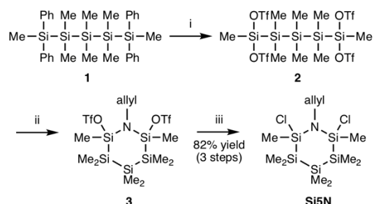
Scheme 1. Synthesis of Si5N . i. TfOH (4 equiv.), pentane; ii. Allylamine (1 equiv.), \text{NEt}_3 (2 equiv.), \text{Et}_2\text{O} . iii. \text{NEt}_3 \cdot \text{HCl} (2 equiv.), \text{Et}_2\text{O}
