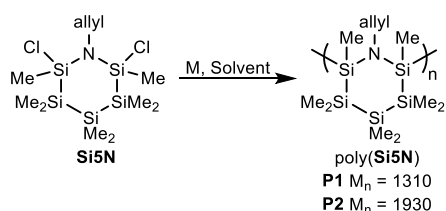
Scheme 2. Generic reductive polymerization of Si5N. P1 was obtained with Na, P2 by Li.
