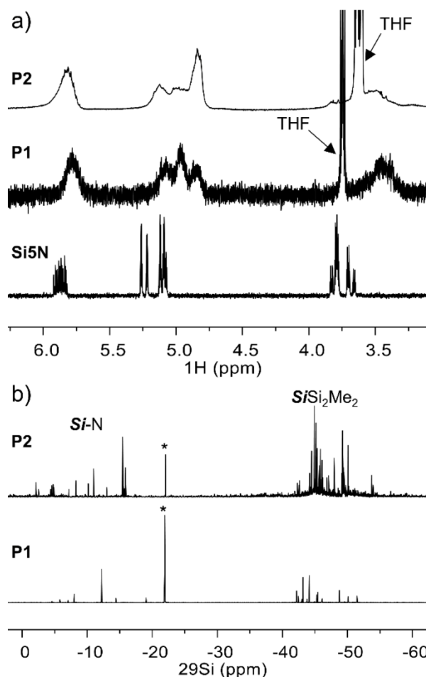
Figure 3. a) Cropped 1 H (400 MHz) NMR spectra of Si5N (CDCl 3 ), P1 (CDCl 3 ), and P2 (THF- d 8 ) and b) Cropped 29 Si ( 1 H) DEPT NMR spectra (79 MHz) of P2 (THF- d 8 ) and P1 (CDCl 3 ). * = silicon grease signal.
