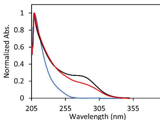
Figure 5. Absorption and spectra of Si5N (blue), P1 (red), and P2 (black). [polymer] = 0.0124 g/L in THF, [ Si5N ] = 1.25 \times 10^{-5} M in THF.
