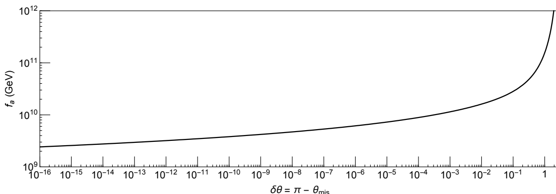
Figure 1. Insensitivity of f_a to very small shifts from the hilltop.
