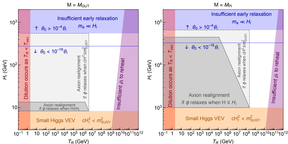
Figure 2. Parameter space for the inflationary Hubble scale H_I and reheate temperature T_R given f_a = 3 \times 10^9 GeV, m_{\tilde{g}} = m_{\text{SUSY}} = \text{TeV} , B\mu = m_{\text{SUSY}}^2 / \tan\beta , \tan\beta = 50 , N_e = 60 , and \phi_i = M . The left (right) panel is for the cutoff scale M = M_{\text{GUT}} ( M_{\text{Pl}} ) respectively.
