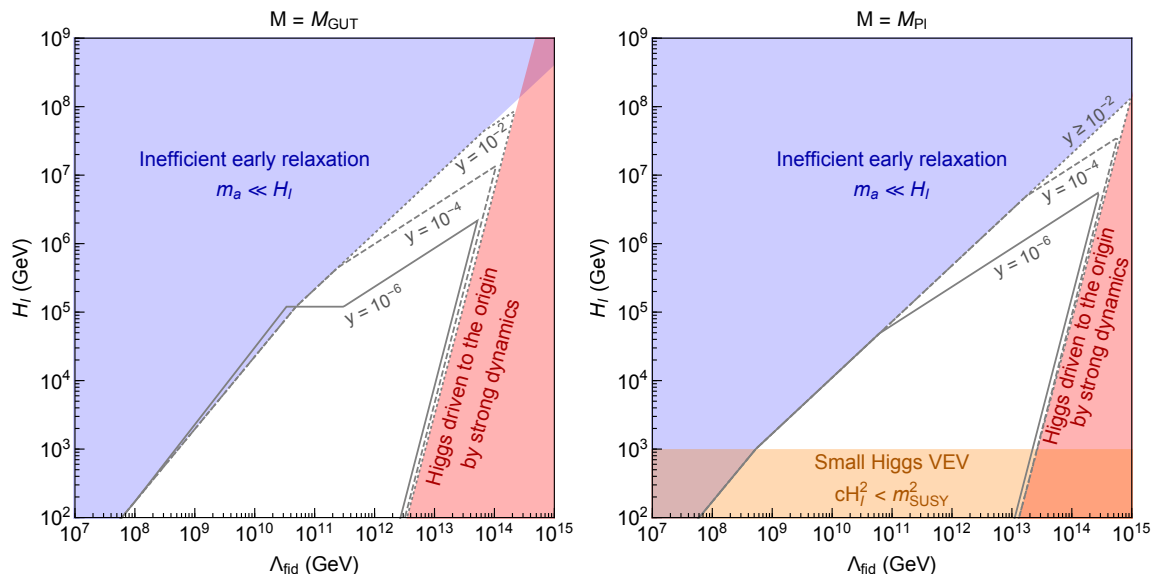
Figure 3. Parameter space for the inflationary Hubble scale H_I and the fiducial confinement scale \Lambda_{\text{fid}} defined in eq. (3.7) given f_a = 3 \times 10^9 GeV, m_{\tilde{g}} = m_{\text{SUSY}} = \text{TeV} , and \phi_i = M . The left (right) panel is for the cutoff scale M = M_{\text{GUT}} ( M_{\text{Pl}} ) respectively.
