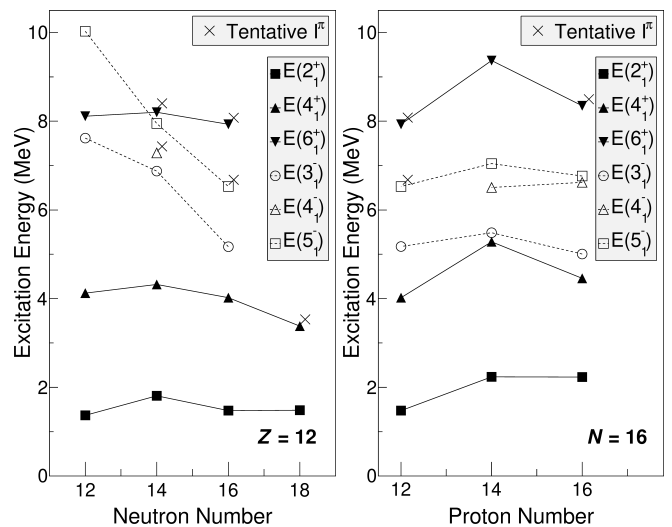
FIG. 5. Left: systematics of known yrast states in Z = 12 isotopes [18, 19, 31, 32]. Right: systematics of known yrast states in N = 16 isotones [19, 20, 33]. Levels from this work which are candidates for the 6_1^+ ( I^\pi = (6^+) , 7929.3(12) keV) and 5_1^- ( I^\pi = (4, 5)^- , 6528.2(9) keV) levels in ^{28}\text{Mg} are shown.
