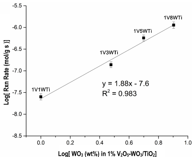
Figure 4. The log [reaction rate] vs log [tungsten oxide loading] (bottom) shows a strong correlation between tungsten oxide content and catalytic performance. Reactions were conducted at 200°C.
