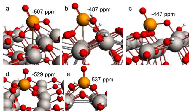
Figure 3. DFT clusters used to model monomeric structures on \text{TiO}_2 , including distorted \text{VO}_4 (a), distorted \text{VO}_4 with bridge bond protonation (b), distorted \text{VO}_4 using two oxygen from \text{TiO}_2 (c), distorted square pyramidal (d), and distorted square pyramidal with bridge bond protonation (e). Atoms represented include vanadium (orange), titanium (grey), oxygen (red), and hydrogen (white).
