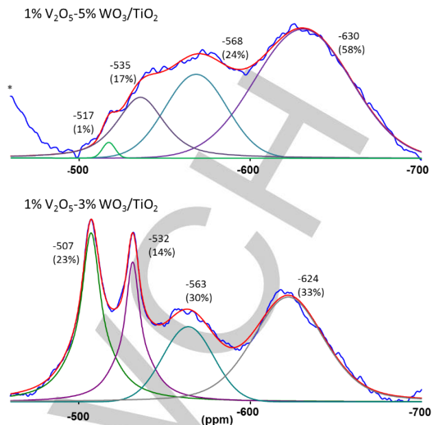
Figure 5. Solid state 51 V MAS NMR spectra of dehydrated, impregnated 1% V 2 O 5 -(3-5)% WO 3 /TiO 2 catalysts. Spectral deconvolution summation is presented by the red line and compared to the collected data (blue). All spectra were externally referenced to V 2 O 5 at -614 ppm. Sidebands displayed are indicated by *.
