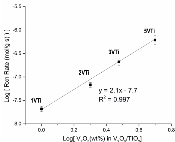
Figure 1. A plot of the log [reaction rate] vs log [vanadium oxide loading] (bottom) reveals a slope of 2, suggesting the preference for two surface vanadia sites in close proximity for the SCR reaction. Reactions were conducted at 200°C.
