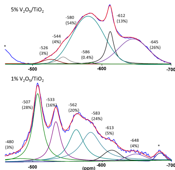
Figure 2. ^{51}\text{V} MAS NMR results of dehydrated, supported \text{V}_2\text{O}_5/\text{TiO}_2 catalysts prepared by impregnation. Spectral deconvolution summation is presented by the red line and compared to the collected data (blue). Sidebands displayed are indicated by (*).
