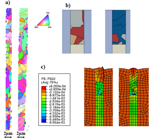
Fig. 6. (a) Grain structure for 2μm TSVs, (b) transcribed grain structure for simulation and (c) resulting plastic strain in the axial direction.
