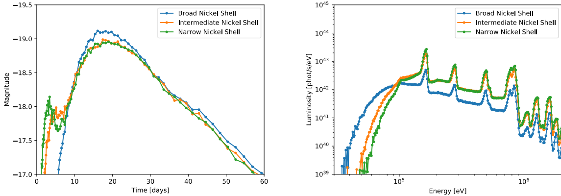
Figure 1: Bolometric light curve (left) and gamma-ray spectra (right) near peak gamma-ray emission for 3 different thermonuclear supernova models. In these models, the explosion energy and nickel production are the same, but the distribution of nickel is altered. Changes in the distribution can significantly alter the gamma-ray signal, ultimately affecting the peak brightness. To truly use thermonuclear supernovae as cosmological tools, we must understand the distribution of nickel production and how it might vary with redshift.
