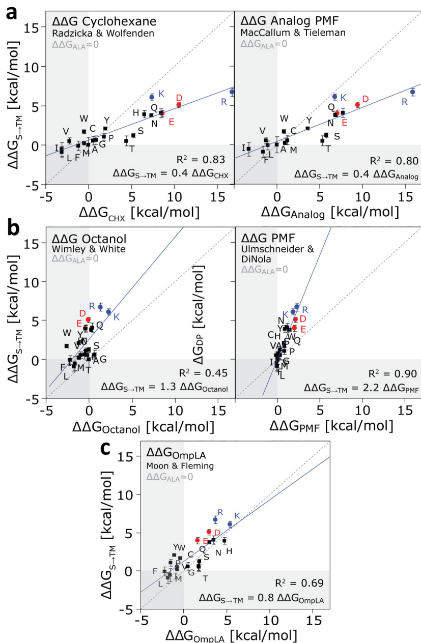
Figure 5. Side-chain only correlations with several experimental and computational scales. Relative free energies (to alanine, \Delta\Delta G_{ALA} = 0 ) are compared as the underlying system in each case is different and absolute comparison of \Delta G_{S \rightarrow TM} not appropriate. (a). Both water-cyclohexane partitioning free energies ( \Delta\Delta G_{CHX} ) of amino acid side chain analogs as well as PMF calculations of sidechain analogs into lipid bilayers ( \Delta\Delta G_{Analog} ) correlate well with \Delta\Delta G_{S \rightarrow TM} , but are scaled up by a factor of \sim 2.5 . These scales lack the contribution of the polar peptide backbone. (b). Whole-residue water/octanol hydrophobicity scales ( \Delta\Delta G_{Octanol} ) derived from small pentapeptides correlate poorly with the simulation data, indicating that peptide water-to-octanol transfer is very different from surface-to-bilayer partitioning. The best correlation is achieved with statistical potentials derived from transmembrane amino acid distributions of membrane proteins of known structure ( \Delta\Delta G_{PMF} ), which are compressed w.r.t. \Delta\Delta G_{S \rightarrow TM} by a factor of 2.2. (c). A similarly good agreement is seen with the recent partitioning experiments using the outer membrane phospholipase A (OmpLA) as a transmembrane scaffold ( \Delta\Delta G_{OmpLA} ). The blue line indicates the best linear fit.
