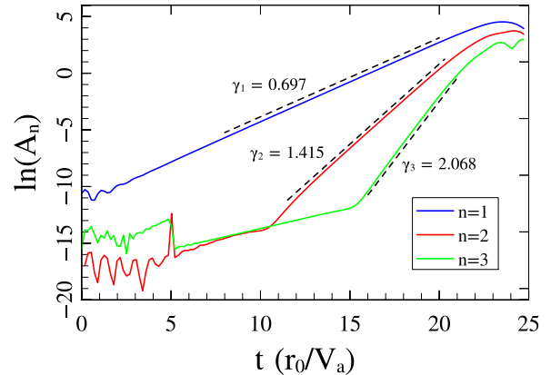
FIG. 2. Time evolution of the three harmonics A_1 , A_2 , and A_3 of the seeded mode with k_z r_0 = 5 and \kappa = 0 . The growth rate at a linear stage is in units of inversed Alfvén time V_a/r_0 .
