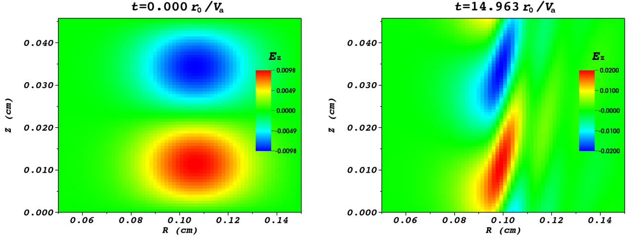
FIG. 4. Evolution of a mode with k_z r_0 = 12.5 , and \kappa = 0.25 . The initial seeded mode tilts and stretches along the axial direction, until it gets to the shape in the right picture, then it slowly grows with the normalized growth rate \gamma \approx 0.081 V_a / r_0 until it get to the nonlinear stage.
