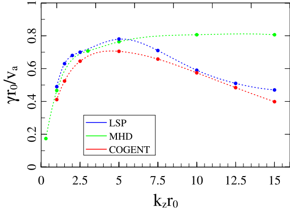
FIG. 3. Normalized growth \gamma of the seeded mode as a function of k_z for no shear flow \kappa=0 . Also comparison to the ideal MHD 27 and kinetic simulations (LSP) 29 .
