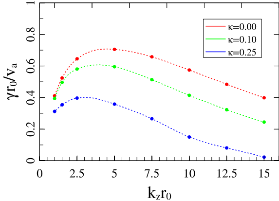
FIG. 6. Normalized growth rate \gamma of the seeded mode as a function of k_z for three values of the shear parameter \kappa . Red: \kappa=0 ; Green: \kappa=0.1 ; Blue: \kappa=0.25 .
