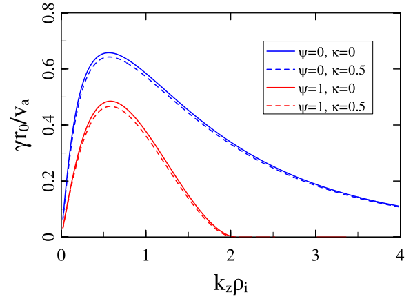
FIG. 1. Normalized growth rate of a local entropy mode at r=r_0 as a function of wave number k_z at k_r=0 for constant ( \psi=0 ) and toroidal ( \psi=1 ) magnetic fields and for two values of the shear parameter. Solid line: no shear \kappa=0.0 ; dashed line \kappa=0.5 .
