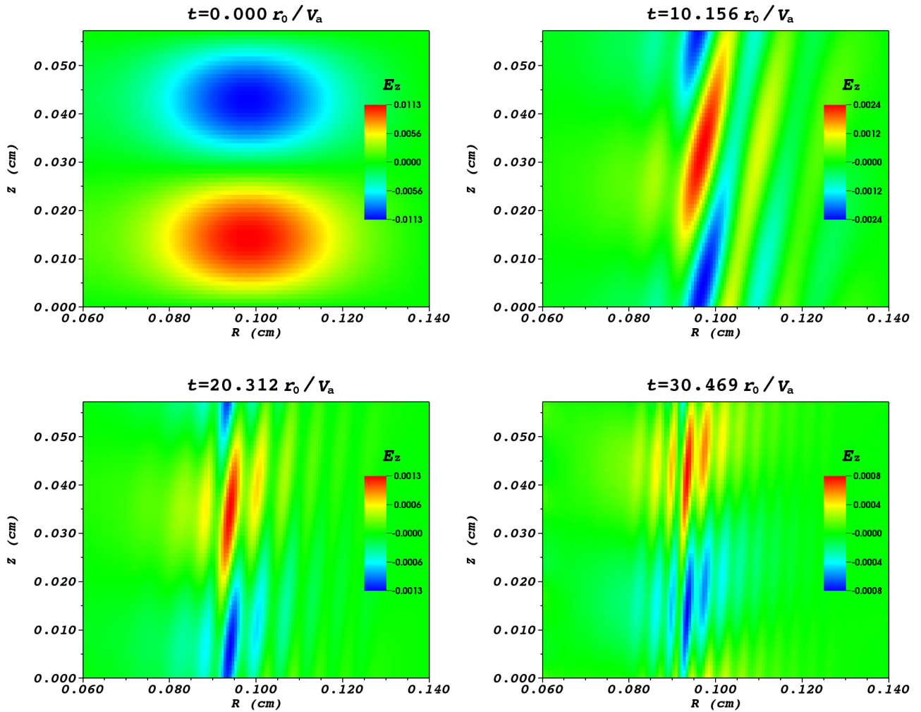
FIG. 5. Evolution of a seeded mode with k_z r_0=10 , and \kappa=0.5 . The initial seeded mode tilts and stretches along the axial direction becoming very narrow in radial direction. Such a structure slowly decays.
