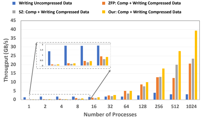
Fig. 8. Throughputs of storing data (compression + I/O) with different solutions on the Hurricane data sets (with the same PSNR).
