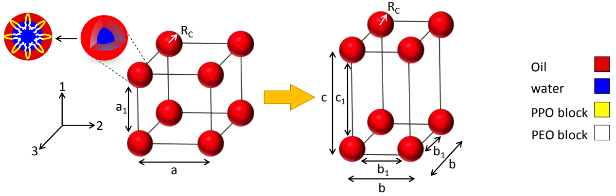
Figure 1. Schematic representation of a micellar cubic mesophase undergoing deformation in direction 1. The legend shows different components in each spherical micelle.
