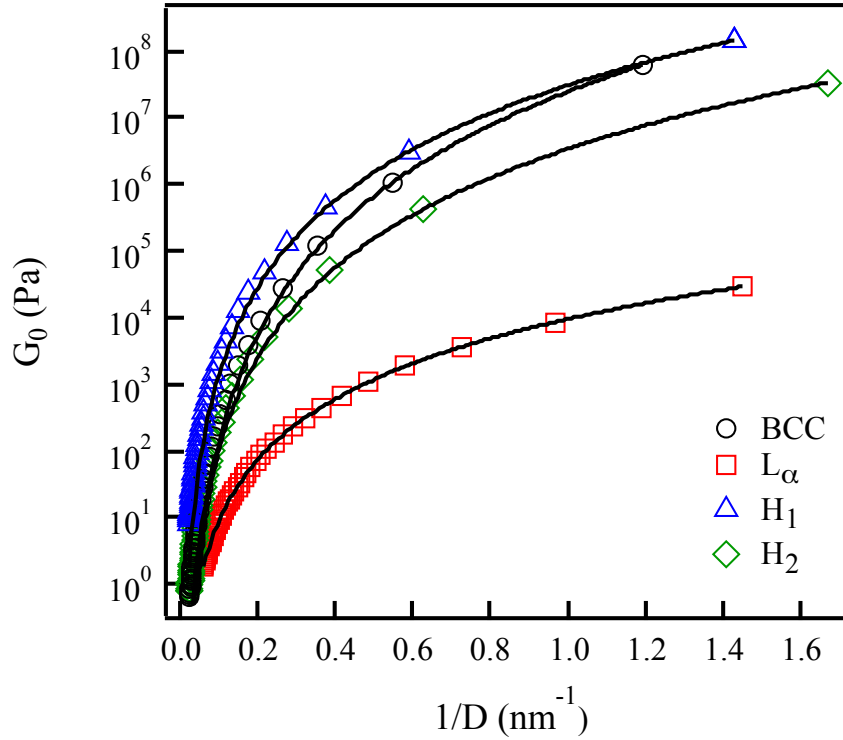
Figure 7. Calculated zero-shear modulus as a function of inverse intermicellar distance ( 1/D ) for micellar cubic, lamellar, normal hexagonal, and reverse hexagonal systems. The solid lines are a power law fit to the data.
