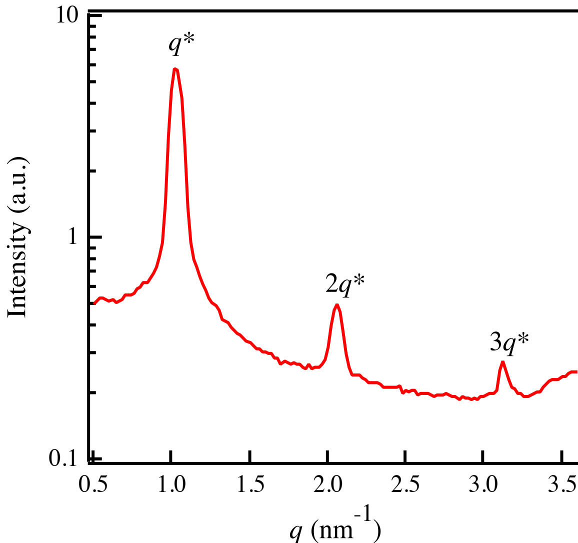
Figure 4. Radially averaged I(q) from SAXS scattering of mesophase systems containing Pluronic P84/water/p-xylene: (a) micellar cubic with 50/10/40 composition, (b) lamellar with 50/35/15 composition, (c) normal hexagonal with 50/47.5/2.5 composition, and (d) reverse hexagonal 50/20/30 composition.
