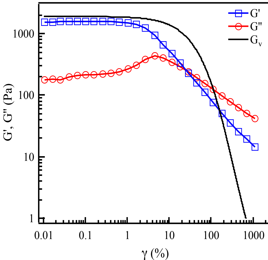
Figure 6. Storage modulus, G' , and loss modulus, G'' , versus strain obtained through amplitude sweep experiments on (a) micellar cubic, (b) lamellar, (c) normal hexagonal and (d) reverse hexagonal mesophases of Pluronic P84/water/p-xylene with 50/10/40, 50/35/15, 50/47.5/2.5, and 50/20/30 compositions, respectively. Solid lines are the estimated shear modulus from the models developed for each mesophase structure.
