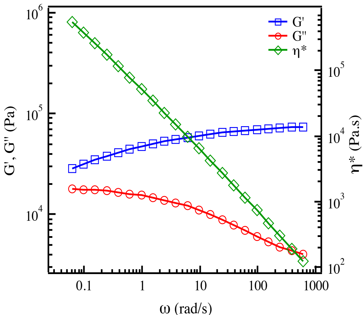
Figure 9. Storage modulus, G' , loss modulus, G'' , and complex viscosity, \eta^* , versus angular frequency obtained through frequency sweep experiments on: (a) micellar cubic, (b) lamellar, (c) normal hexagonal, and (d) reverse hexagonal mesophases of Pluronic P84/water/p-xylene with 50/10/40, 50/35/15, 50/47.5/2.5, and 50/20/30 compositions, respectively.
