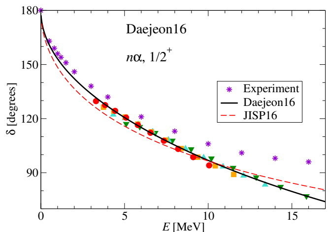
FIG. 21. Non-resonant n\alpha scattering in the \frac{1}{2}^+ state with the Daejeon16 NN interaction in comparison with that obtained with JISP16 in Ref. [32]. Experimental data (stars) are taken from Ref. [69]. See Fig. 3 for other details and Fig. 20 for the correspondence of the symbols to the NCSM calculations with various N_{\text{max}} values.
