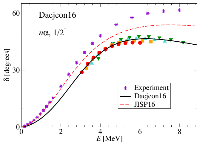
FIG. 15. n\alpha scattering in the \frac{1}{2}^- states with the Daejeon16 NN interaction in comparison with that obtained with JISP16 in Ref. [32]. Experimental data (stars) are taken from Ref. [69]. See Fig. 3 for other details.
