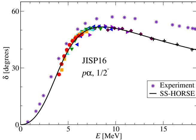
FIG. 8. p\alpha scattering in the \frac{1}{2}^- state with the JISP16 NN interaction. See Fig. 3 for details.
