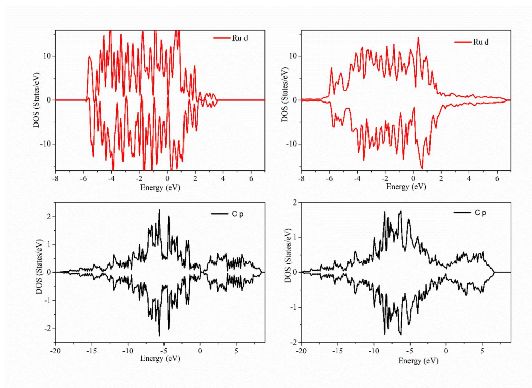
Fig. 10. Projected density of states (PDOSs) of the d orbitals of \text{Ru}_{13} (upper panels) and the p orbitals of interfacial carbons in the CNT (lower panels). The left column (a and c) is for individual \text{Ru}_6 and CNT while the right column (b and d) is for the combined system. The Fermi level is set to 0 eV.
