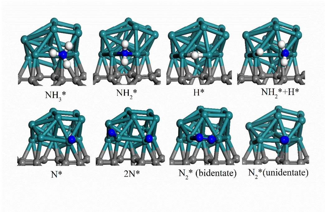
Fig. 5. Adsorption geometries of pertinent species on interfacial sites of Ru 13 @CNT.
