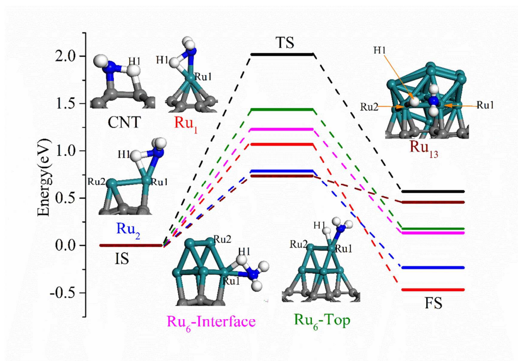
Fig. 6. Reaction paths of \text{NH}_3^* \rightarrow \text{NH}_2^* + \text{H}^* on CNT (black line), \text{Ru}_1@\text{CNT} (red line), \text{Ru}_2@\text{CNT} (blue line), interfacial sites of \text{Ru}_6@\text{CNT} (magenta line), top layer sites of \text{Ru}_6@\text{CNT} (olive line) and \text{Ru}_{13}@\text{CNT} (wine line). The geometry of transition states (TS) are also given. The geometries of initial state (IS) and final state (FS) are referred to the corresponding geometries of \text{NH}_3 and \text{NH}_2 + \text{H} shown in Figs 3-5. The same color scheme as Fig. 3 is used.
