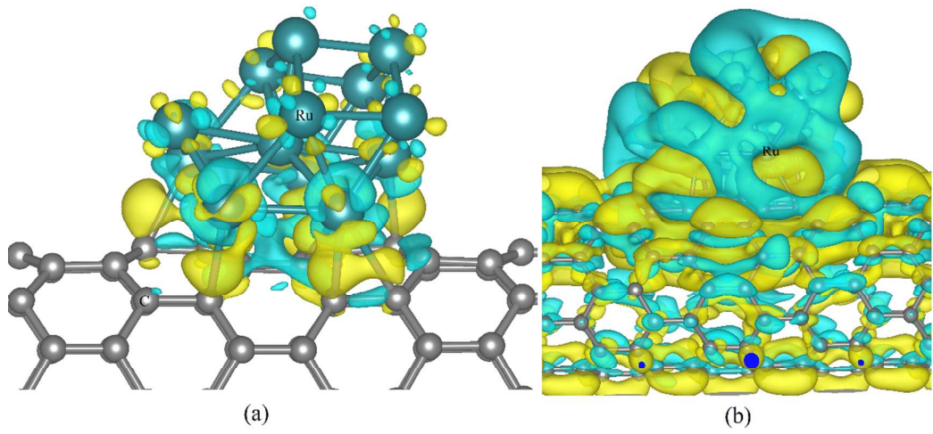
Fig. 9. Contour plots of the differential charge density of Ru 13 @CNT. The charge accumulation region is rendered in blue while the charge depletion region in yellow. The isosurface level is \pm 0.005 and \pm 0.00008 au for (a) and (b), respectively. Color code: C, gray; Ru, cyan.
