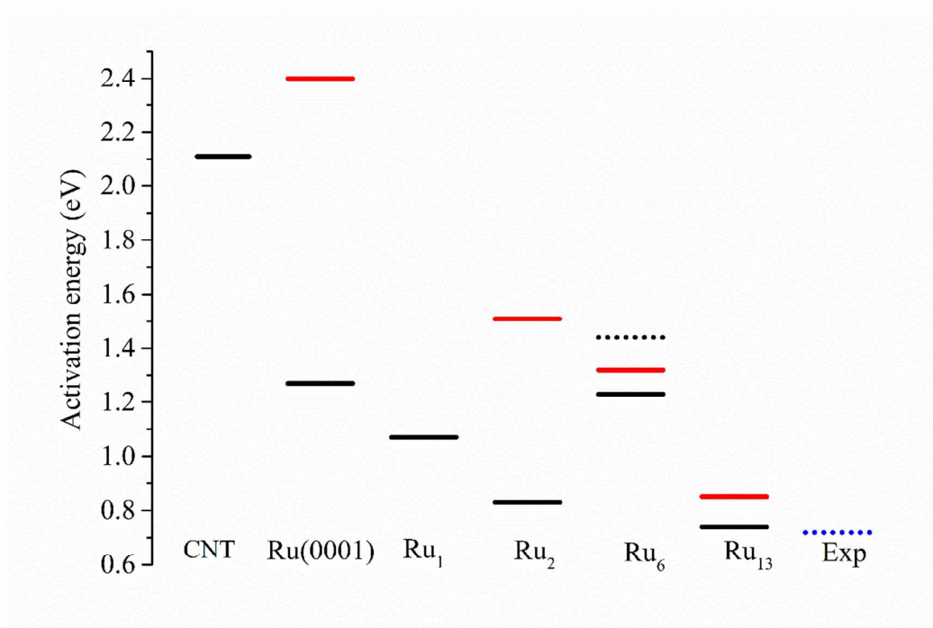
Fig. 8. Size dependence of the activation energy for ammonia dehydrogenation (reaction (1)) and nitrogen recombination (reaction (5)). Solid black line: reaction (1); Solid red line: reaction (5). Here Ru x ( x=1, 2, 6 and 13 ) indicates the corresponding Ru x @CNT. For Ru 6 @CNT, the solid lines give the results on the interface while black dot line displays the results of reaction (1) on top layer sites. The DFT results on Ru(0001) are also given, while the blue dotted line indicates the experimental apparent activation energy.
