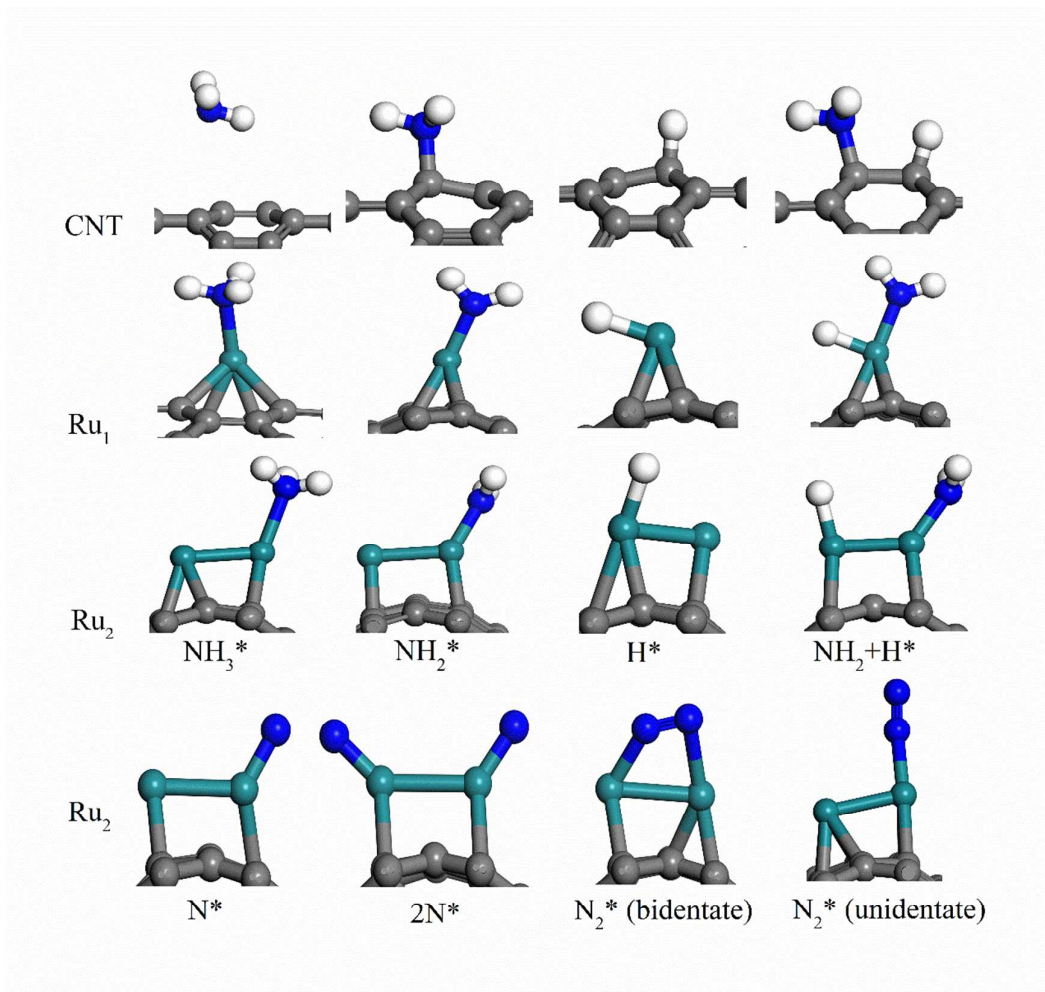
Fig. 3. Adsorption geometries of pertinent species on CNT, \text{Ru}_1 @CNT, and \text{Ru}_2 @CNT. The C, Ru, N, and H atoms are colored in gray, cyan, blue, and white, respectively.
