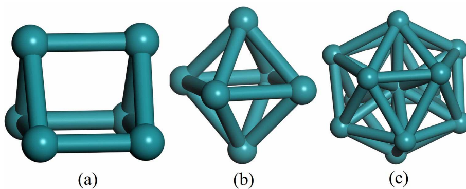
Fig. 2. Geometries of isolated Ru 6 (a and b) and Ru 13 (c).
