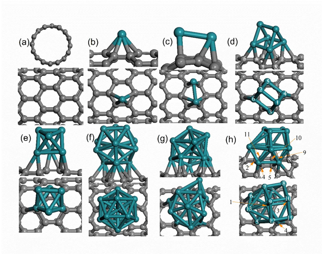
Fig. 1. Side and top views of the geometries of CNT (a), Ru 1 @CNT (b), Ru 2 @CNT (c), Ru 6 @CNT (d and e) and Ru 13 @CNT (f-h). The C and Ru atoms are colored in gray and cyan, respectively.
