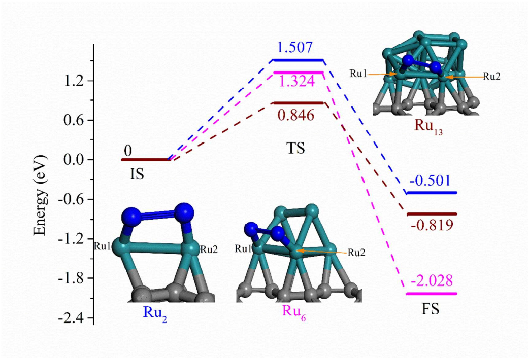
Fig. 7. Calculated reaction paths of N 2 formation on Ru 2 @CNT (blue line), Ru 6 @CNT (magenta line) and Ru 13 @CNT (vine line). The geometry of transition states is also given. The geometries of initial state (IS) and final state (FS) are referred to the corresponding geometries of 2N* and N 2 * shown in Figs. 3-5. The same color scheme as Fig. 3 is used.
