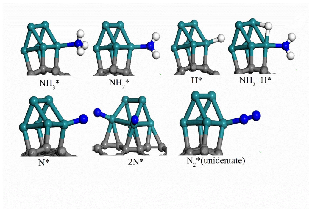
Fig. 4. Adsorption geometries of pertinent species on interface layer of Ru 6 @CNT.
