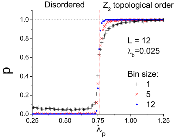
FIG. 9. The ratio of ‘topological’ response as a function of \lambda_p at fixed \lambda_b = 0.025 . The neural network is prepared with training set using \lambda_p = 1.25 for the topological phase ( y = 1 ) and \lambda_p = 0.25 for the trivial (disordered) phase ( y = 0 ), and then applied to the phase space in between. The decision is based upon the criteria that average neural output \bar{y} > 0.5 over a number of uncorrelated samples. The vertical red dashed line at \lambda_p = 0.76 is the approximate location of the transition.
