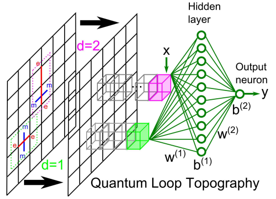
FIG. 1. Schematic illustration of our machine learning architecture. Quantum loop topography uses an ensemble of ‘minimally non-local’ operators to extract information from the many-body systems and creates ‘image’ with relevant information for the input into the artificial neural network.
