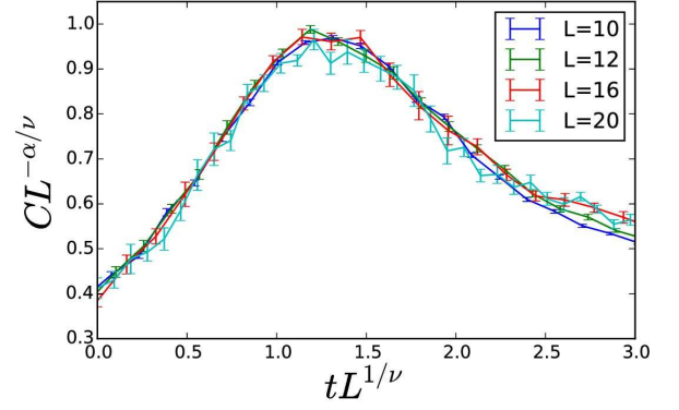
FIG. 5. Specific heat data of the three-dimensional system H_{3D} from Eq. 5 for a range of system sizes L = 10, 12, 16, 20 is collapsed according to the finite-size scaling using critical exponents of the three-dimensional Ising universality class. The best collapse is achieved at critical temperature k_B T_c = 1.324(1) for \lambda_p/\beta = 1 and \lambda_b/\beta = 0.29 .
