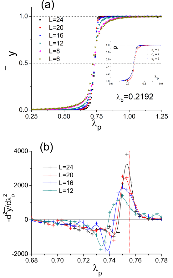
FIG. 8. (a) The neural output \bar{y}(\lambda_p) over the range 0.25 \leq \lambda_p \leq 1.25 . (b) The second derivative -d^2 \bar{y} / d \lambda_p^2 in the critical region 0.68 \leq \lambda_p \leq 0.78 from higher-resolution data. \bar{y} is averaged over 20000 Monte Carlo samples at \lambda_b = 0.2192 and different system sizes L . Inset: The ratio of topological response ‘p’ for different QLT cut-off d_c = 1, 2, 3 at L = 12 . The red dashed lines mark the location of the transition \lambda_p = 0.7553 obtained using specific heat collapse, see Fig. 5.
