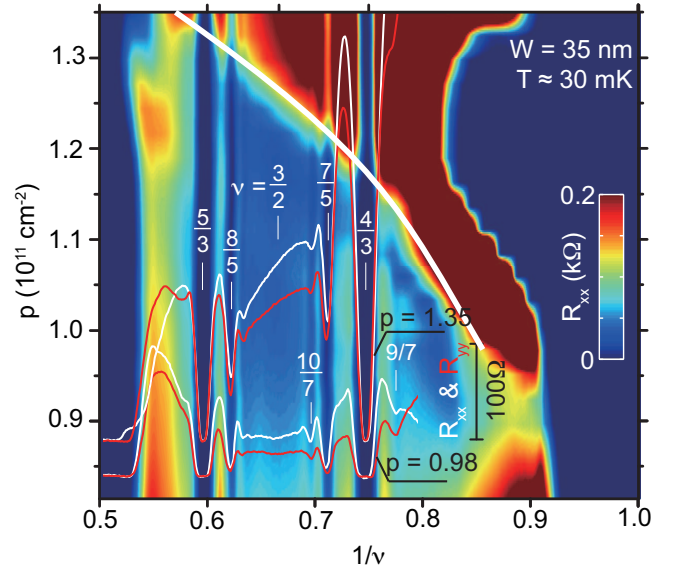
FIG. 2. (color online) Color-coded plot of R_{xx} measured from the 35-nm-wide QW sample at \theta = 0^\circ and different densities. A sharp phase transition can be seen as a steep increase of R_{xx} at the boundary marked by the solid white line, signaling a LL crossing. The R_{xx} (white) and R_{yy} (red) traces are taken at p = 0.98 and 1.35 \times 10^{11} \text{ cm}^{-2} , before and after the crossing, respectively. Despite the significant increase in R_{xx} and R_{yy} , the 2DHS in both cases is isotropic and exhibits strong FQHSs at \nu = 4/3, 5/3 , etc., and a compressible Fermi sea at \nu = 3/2 , indicating the two crossing LLs are both N = 0 .
