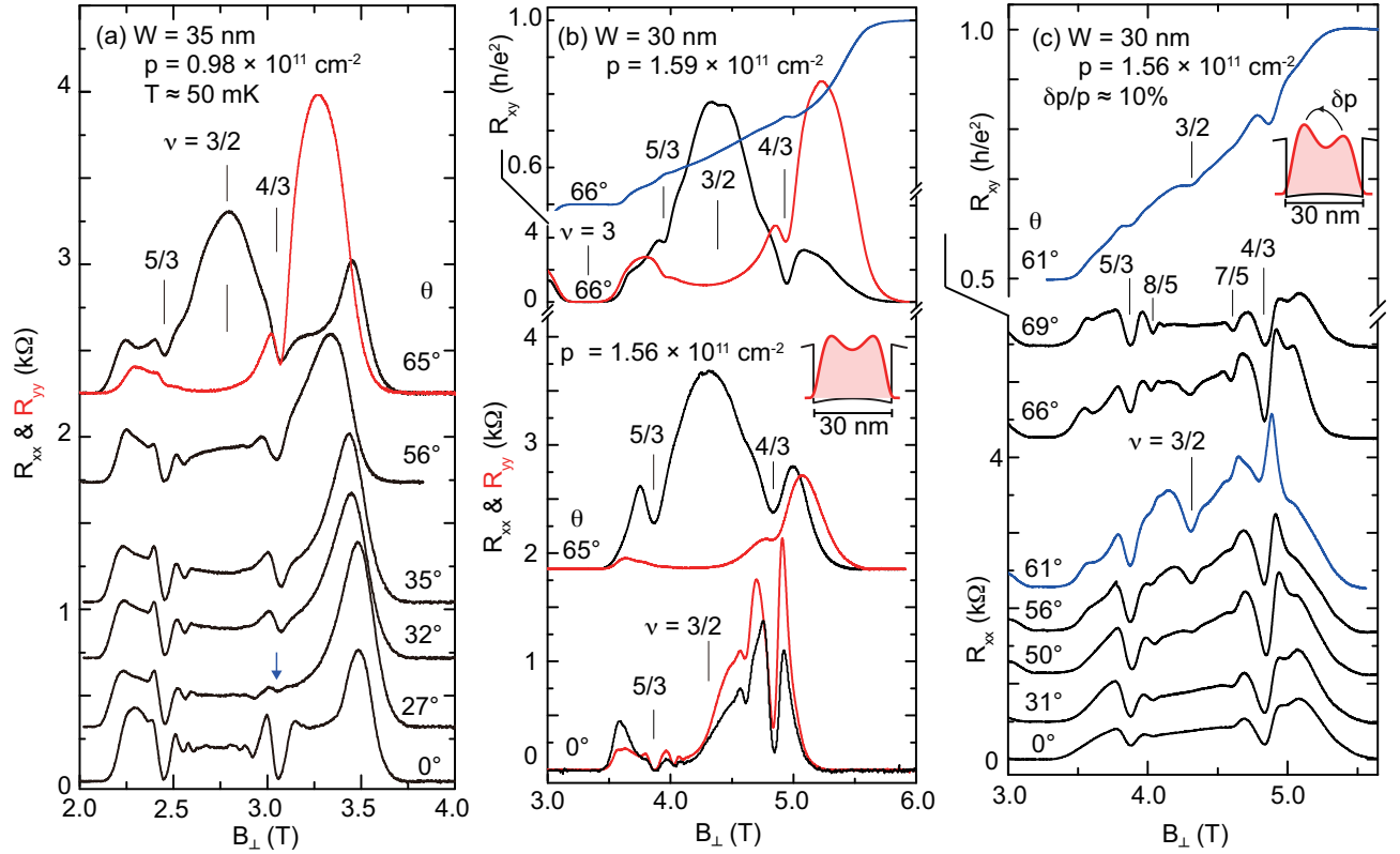
FIG. 3. (color online) (a) R_{xx} and R_{yy} for the 35-nm-QW 2DHS at density p \approx 0.98 \times 10^{11} \text{ cm}^{-2} and different tilt angles ( \theta ). At \theta = 65^\circ , the compressible Fermi sea at \nu = 3/2 turns into a stripe phase and the R_{xx} minima at \nu = 4/3 and 5/3 become weak. (b) Magneto-resistances for the symmetric 30-nm-QW samples. (c) In a slightly asymmetric QW, no stripe phase but a Fermi sea is seen at very large \theta . Remarkably, near \theta \approx 61^\circ , an even-denominator FQHS is seen at \nu = 3/2 . In all panels, the traces are shifted vertically for clarity.
