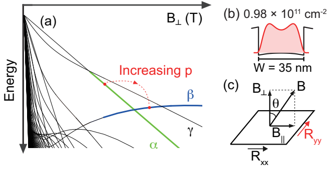
FIG. 1. (color online) (a) Schematic LL diagram. The light-hole-like \beta -level (blue) crosses the heavy-hole-like \alpha -level (green) as a function of B_{\perp} . As indicated by the red arrow, the Fermi energy E_F at \nu = 3/2 moves from the \alpha - to the \beta -level as we increase the density. (b) Calculated charge distribution and potential of the 35-nm-QW 2DHS at p = 0.98 \times 10^{11} \text{ cm}^{-2} . (c) Measurement setup. B_{\parallel} is applied by tilting the sample in field, and R_{xx} and R_{yy} denote the longitudinal resistance measured along and perpendicular to B_{\parallel} .
