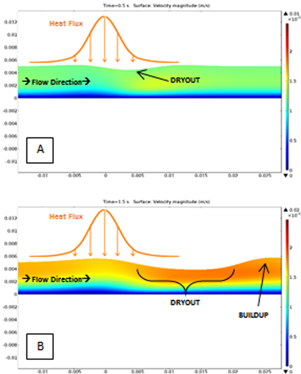
Fig. 3.5. A) The beginning of the lithium depression as dryout begins and is propelled downstream by lithium flow. B) Developed dryout phenomenon under high heat flux exhibits pronounced lithium depression and lithium buildup downstream. Distance is in meters and velocity values are in meters per second.
