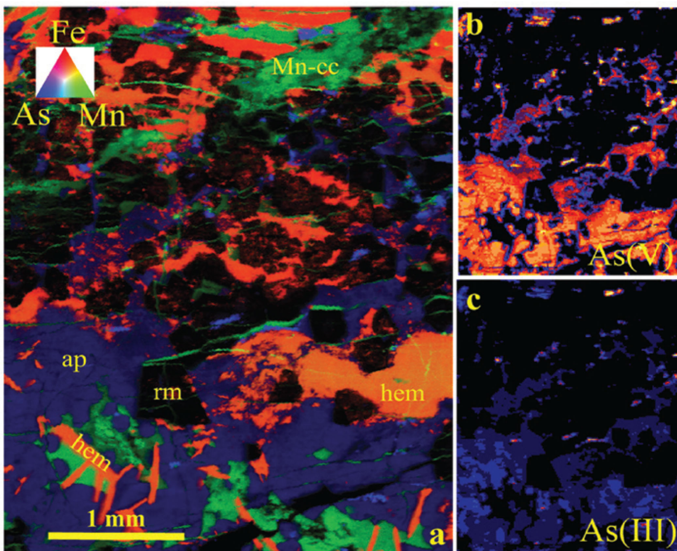
Fig. 11: Imaging of a Fe-Mn ore sample. (a) SXRf 2.112 million pixel RgB image built from the Fe, As, and Mn quantitative elemental maps ( 12.3892 \text{ keV} ; 3.3 \times 4 \text{ mm}^2 ; 1.25 \times 5 \mu\text{m} resolution; moving the sample stage with a velocity of 4.7 \text{ mm/s} . (b and c) XANES images, smoothed with a boxcar filter over (20,4) pixels. Maximum concentrations (wt%): Fe = 65.7; As = 26.18; Mn = 29.8. ap = apatite, Mn-cc = Mn-calcite, hem = hematite, rm = roméite [64].
