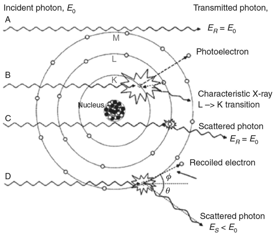
Fig. 1: Interaction processes of X-rays with matter.
