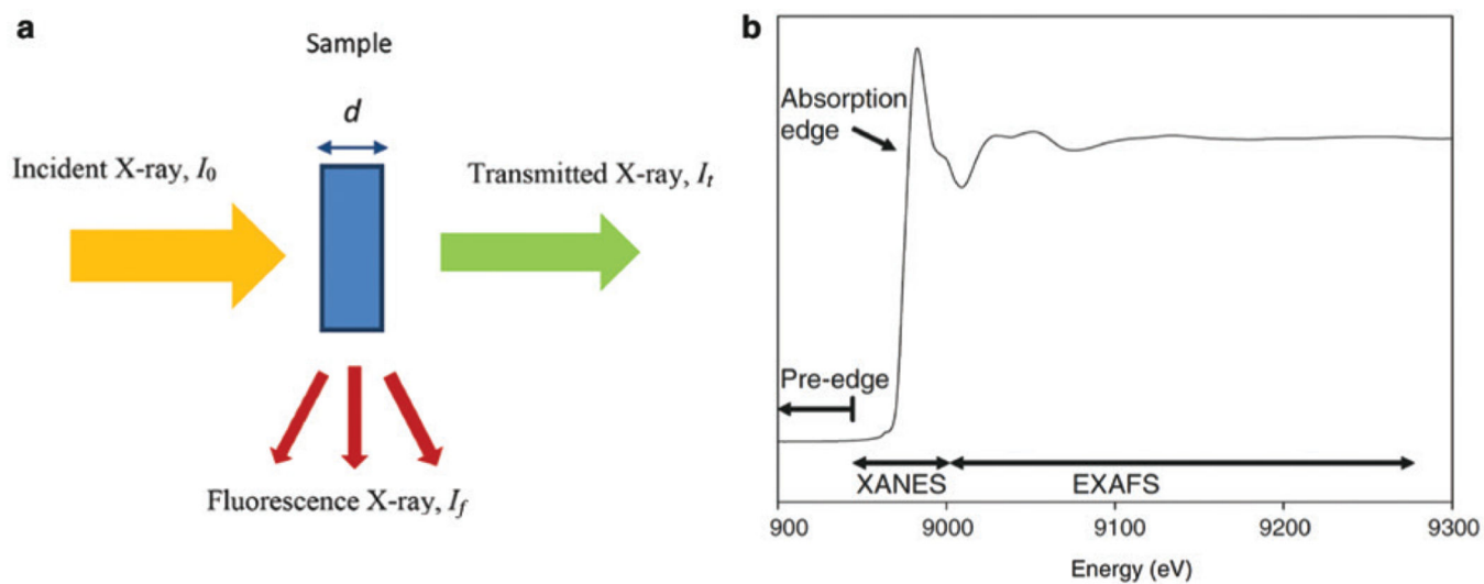
Fig. 4: (a) Experimental arrangement for X-ray absorption spectroscopy (b) Cu K XAS spectrum of malachite [ \text{CuCO}_3 \cdot \text{Cu}(\text{OH})_2 ] showing the region of the spectrum pertinent to XANES and EXAFS.
