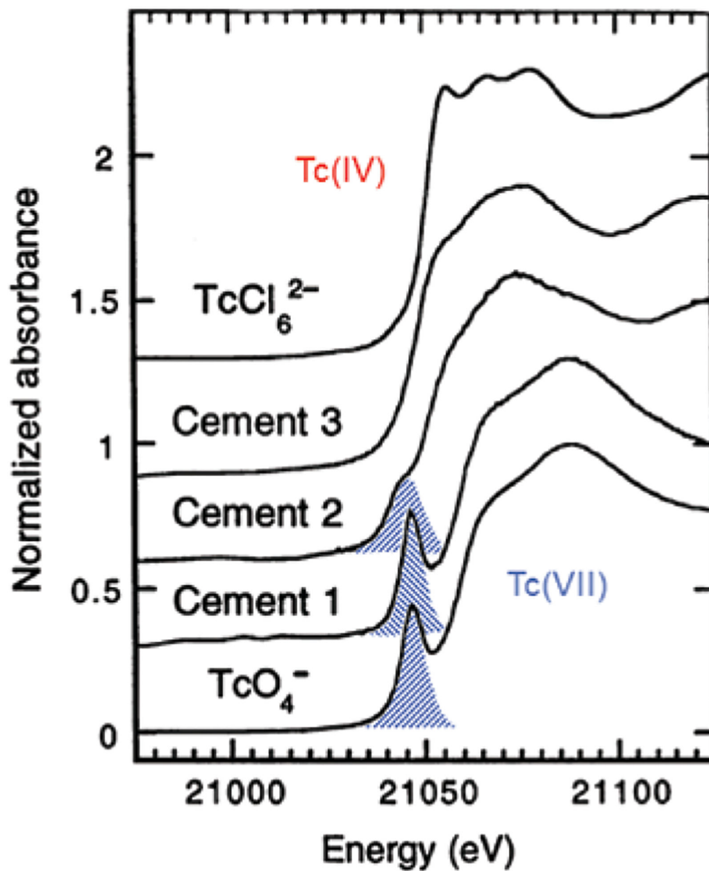
Fig. 5: Technetium K XANES measured for cement samples containing tetraoxidotechnetate(VII) without additives (Cement 1), added blast-furnace slag for partial reduction (Cement 2) and added \text{Na}_2\text{S} for complete reduction (Cement 3), compared to known reference compounds containing technetium(IV) (top) and technetium(VII) (bottom).
