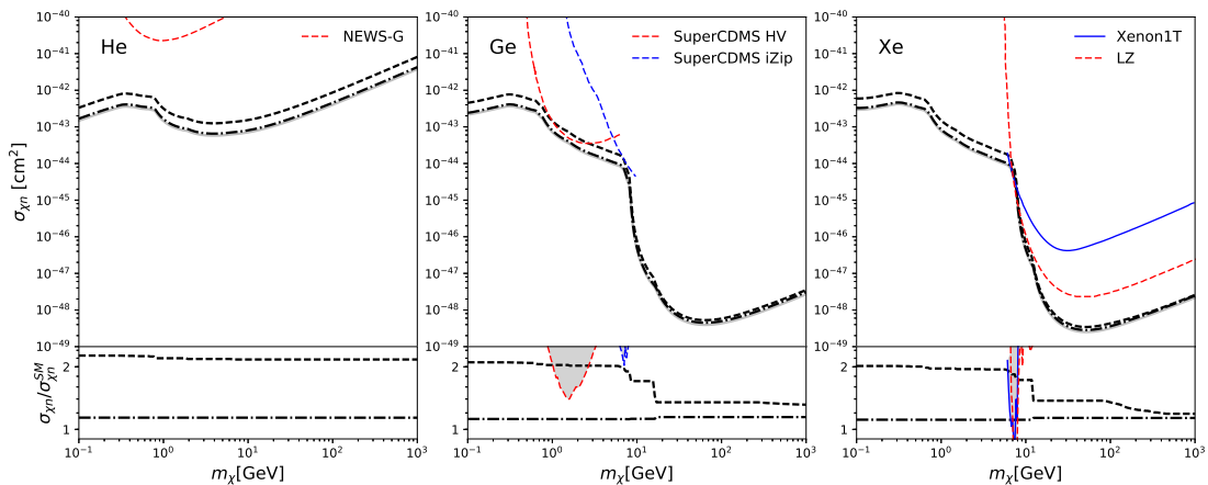
FIG. 2. Upper: CE \nu NS floor for a new vector mediator, computed for direct detection experiments utilising, from left to right, He, Ge, and Xe. The SM neutrino floor (solid, grey) is compared with the maximum level reached in a B-L (dashed, black) and a B-L(3) (dot-dashed, black) model. For comparison, the sensitivities of some current (solid) and future (dashed) direct detection experiments are shown in color. Lower: Ratio of the new neutrino floor to the SM result. The sensitivities of representative direct detection experiments are also shown in this parameter space.
