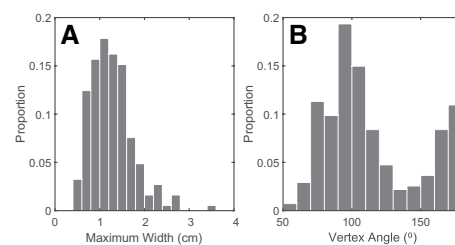
Figure 3. Distribution of the maximum width of polygons (A) and vertex angles (B) formed by ridges on Old Soaker rock slab, Mars.
