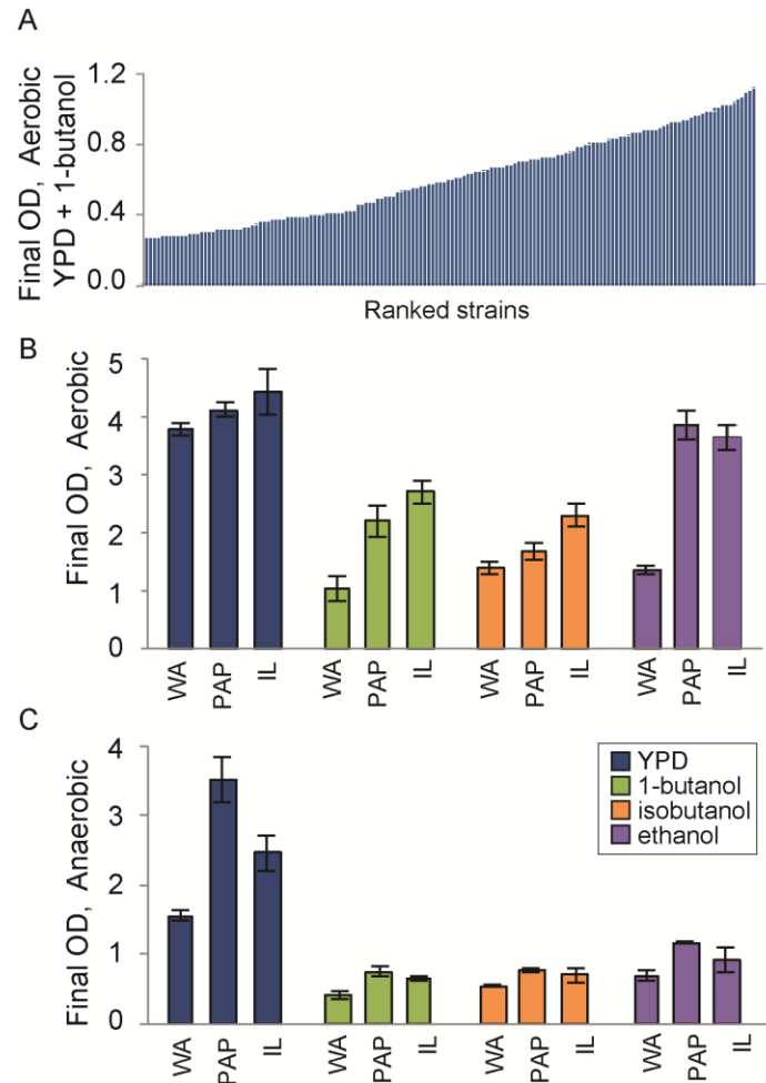
Figure 1. Strain-specific tolerance of alcohols varies with oxygen. (A)
