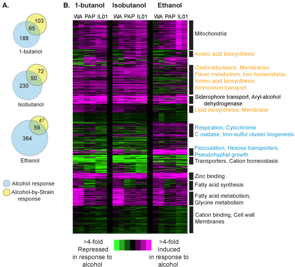
Fig 3. Expression responses to butanol, isobutanol, and ethanol in aerobic conditions. (A) Venn diagrams represent the number of genes whose expression responds to alcohol independent of strain and genes with a strain-specific response, for each alcohol. (B) Hierarchical clustering of 776 genes identified as differentially expressed in response to 0.8% butanol, 1% isobutanol, or 4% ethanol compared to YPD, in cells growing aerobically. Genes were clustered based on the \log_2 (fold change) in expression in each strain (WA, PAP, IL) grown in the indicated alcohol versus YPD, in biological duplicate. Expression changes are colored to indicate induction (pink) and repression (green) according to the key. Functional categories enriched in each cluster ( p < 1e-4 , FunSpec) are shown to the right of each cluster. Responses specific to ethanol are highlighted in blue text and those specific to butanols are highlighted in orange text.
