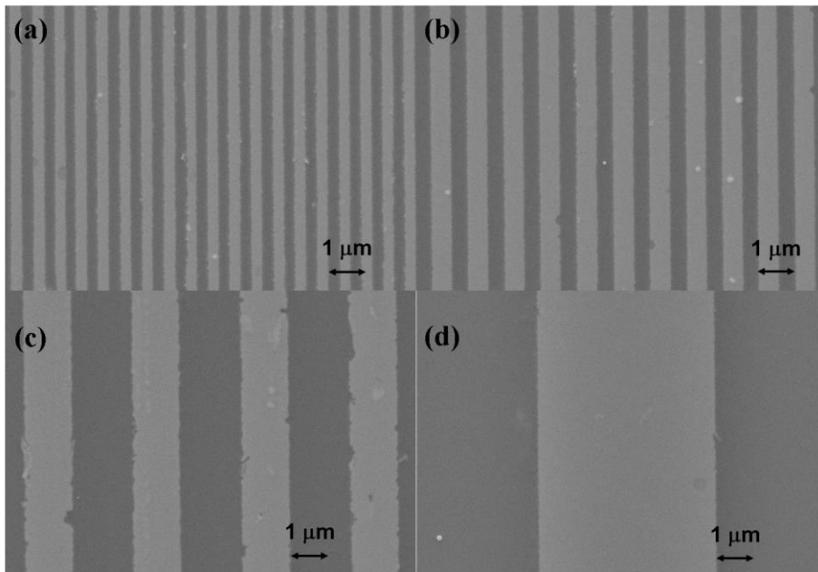
FIG. 1. SEM images at the same magnification of the multi-element antennas on a YIG film with periods of: (a) 0.6 \mu\text{m} , (b) 1 \mu\text{m} , (c) 3 \mu\text{m} , and (d) 10 \mu\text{m} .
