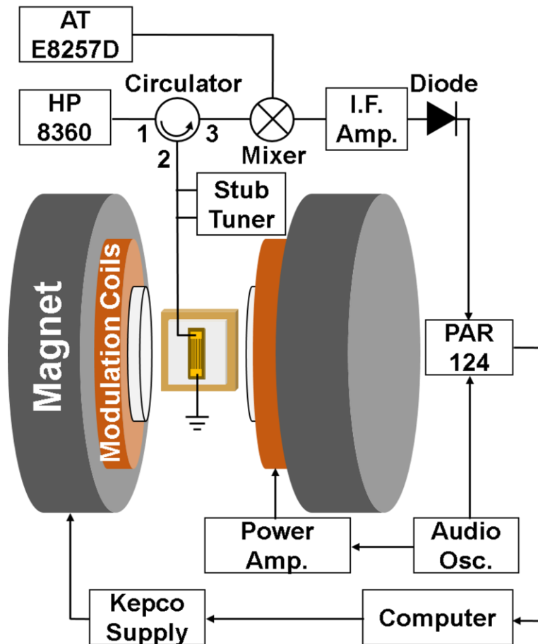
FIG. 2. A schematic of the FMR measurement system. A 200 \mu\text{m} thick glass cover slip creates a gap between the YIG film and the Cu base plate of the sample holder to avoid any effects from an adjacent conducting surface.
