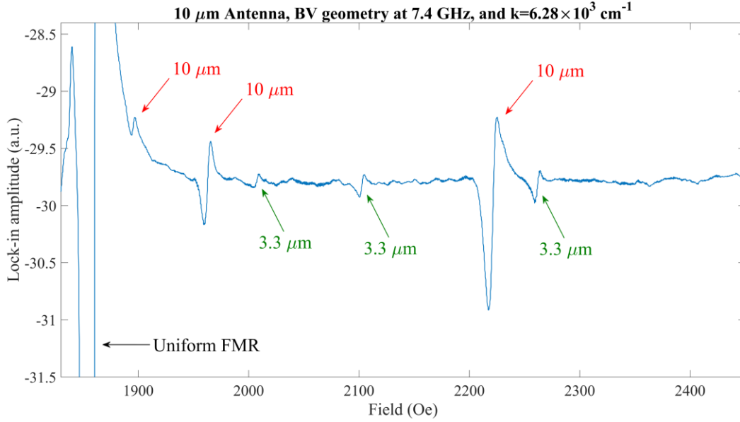
FIG. 3. An example of raw data generated from a 10 \mu\text{m} period antenna. There are three classes of signals. The first, which is off-scale, arises from the uniform precession mode (FMR), the second is caused by the three lowest lying BV modes having an in-plane wavelength of 10 \mu\text{m} , while the last is from the corresponding three BV spin waves with an in-plane wavelength of 3.3 \mu\text{m} generated from first odd spatial sub harmonic ( n = 3 ) of the antenna.
