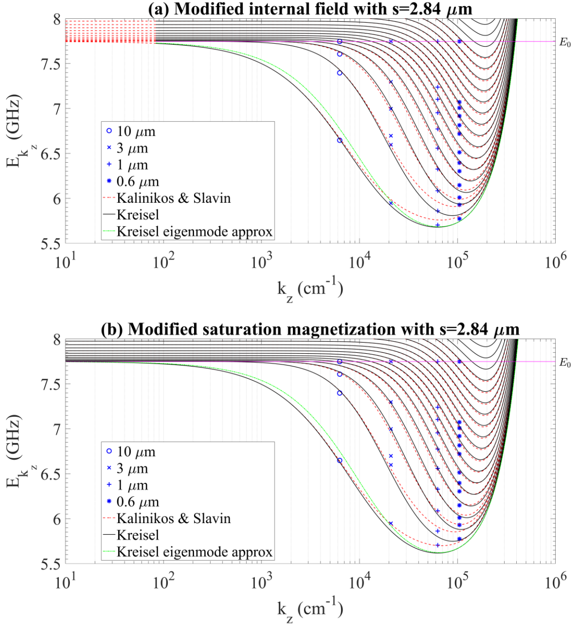
FIG. 4. The measured frequencies of the lowest lying, and the first few exchange split, backward volume spin waves in a 2.84 \mu\text{m} thick YIG film at wavelengths of 10 , 3 , 1 and 0.6 \mu\text{m} . Shown also are the microscopic calculations involving the model spin Hamiltonian (black solid line) together with an approximate treatment based on a Fourier expansion of the magnetostatic Landau-Lifshitz equation (red dashed line). 4(a) shows the comparison using a modified internal field while 4(b) shows that for a modified saturation magnetization. Also shown is an approximate treatment due to Kreisel et. al. (green dot-dashed line). Finally, the line on the line designated E_0 correspond to the k = 0 (uniform) FMR mode.
