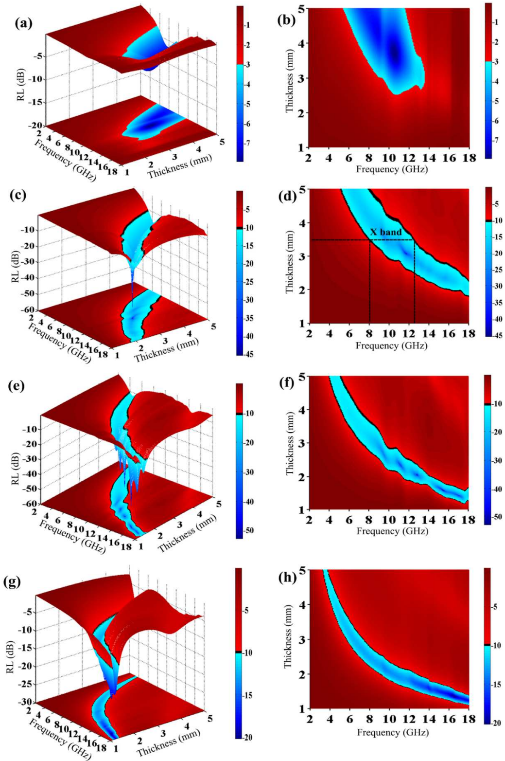
Fig. 4. 3D representations of RL values (a, c, e and g) and corresponding 2D contour plots (b, d, f, h) for sample (a, b) F5, (c, d) F6, (e, f) F7 and (g, h) F8.
