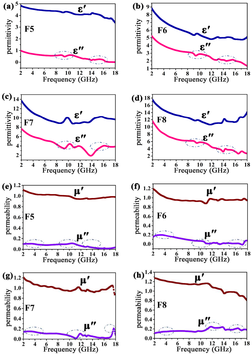
Fig. 3. Frequency dependence of complex permittivity for sample (a) F5, (b) F6, (c) F7 and (d) F8; frequency dependence of complex permeability for sample (e) F5, (f) F6, (g) F7 and (h) F8.
