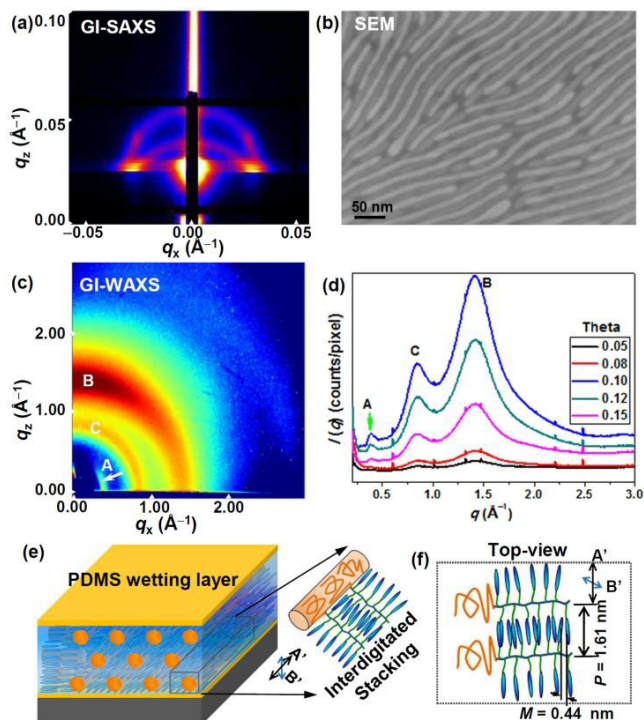
Fig. 4 (a) 2D GISAXS pattern with incident angle 0.15^\circ of the 140 nm thick BCP film after annealing at 120^\circ\text{C} ; (b) a representative SEM image of oxidized PDMS cylindrical nanopatterns formed in the thin film; (c) 2D GIWAXS pattern with incident angle 0.15^\circ , and (d) the 1D GIWAXS profiles with incident angle from 0.05^\circ to 0.15^\circ . (e, f) schematic illustrations of the in-plane cylinder with LC mesogens in a smectic LC phase, where the mesogen \pi - \pi interaction direction is perpendicular to the smectic layer direction.
