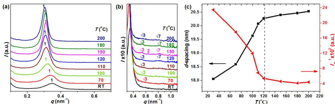
Fig. 3 (a,b) SAXS profiles measured in situ during annealing of PDMS- b -P(4CNB11C)MA BCP. (c) the d -spacing values (black squares) and the reciprocal of the maximum scattering intensity of the primary scattering peak (red triangles) as a function of the temperature.
