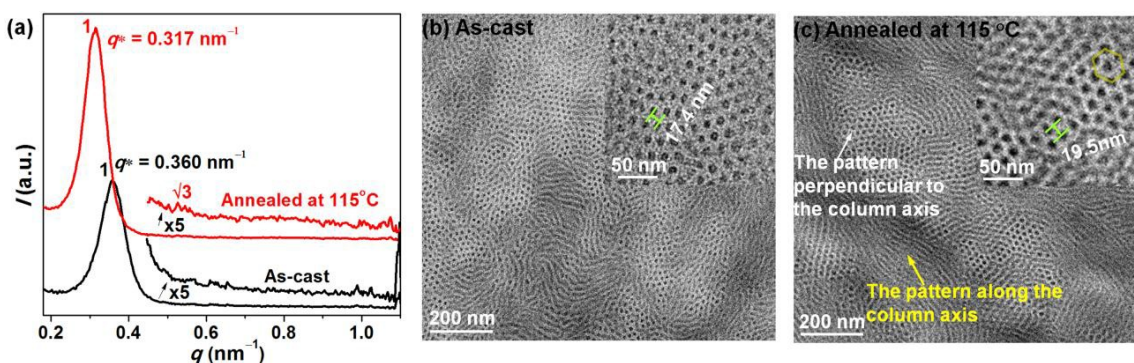
Fig. 2 (a) SAXS profiles of the PDMS- b -P(4CNB11C)MA as-cast (black curve) and after annealing at 115 °C (red curve); and the TEM images of sample after drying from solution (b) and after thermal annealing at 115 °C (c) with the insets showing higher magnification images. The area indicated by the yellow arrow indicates microdomains sectioned along the hexagonal column direction and that indicated by the white arrow indicates microdomains perpendicular to the column axis of the HEX structure.
