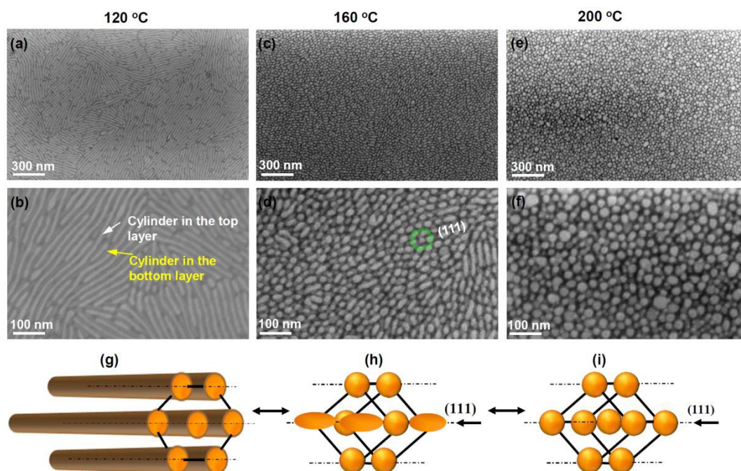
Fig. 6 SEM images of oxidized PDMS patterns from the thin films of PDMS- b -P(4CNB11C)MA BCP quenched from (a,b) 120 °C, (c,d) 160 °C and (e,f) 200 °C, and (g–i) a schematic illustration of the HEX to BCC transition.
