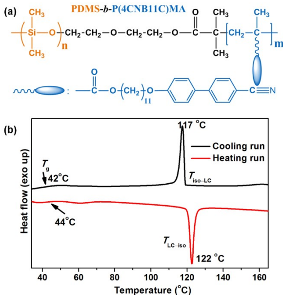
Fig. 1 The chemical structure of PDMS- b -P(4CNB11C)MA side chain LC block copolymer (a), and the DSC curves of this BCP in the second heating scan (red) and in the second cooling scan (black) with a scanning rate of 10 °C/min.
