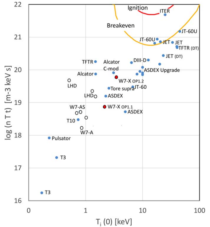
Figure 16. Triple products versus ion temperatures are shown for a variety of experiments. The results from OP1.1 and OP1.2 in W7-X are shown in red, and compared to tokamaks (blue) and stellarator/heliotron experiments (empty circles). All are achieved values except for ITER, under construction, for which we have taken a recent prediction for the Q = 10 scenario [48].
