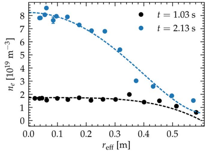
Figure 13. The density profiles before pellet injection and around the time of the record triple product (shortly after pellet injection stopped) are shown. The density went up strongly during pellet fueling and there was a pronounced central peaking. The data were measured with a Thomson scattering system.
