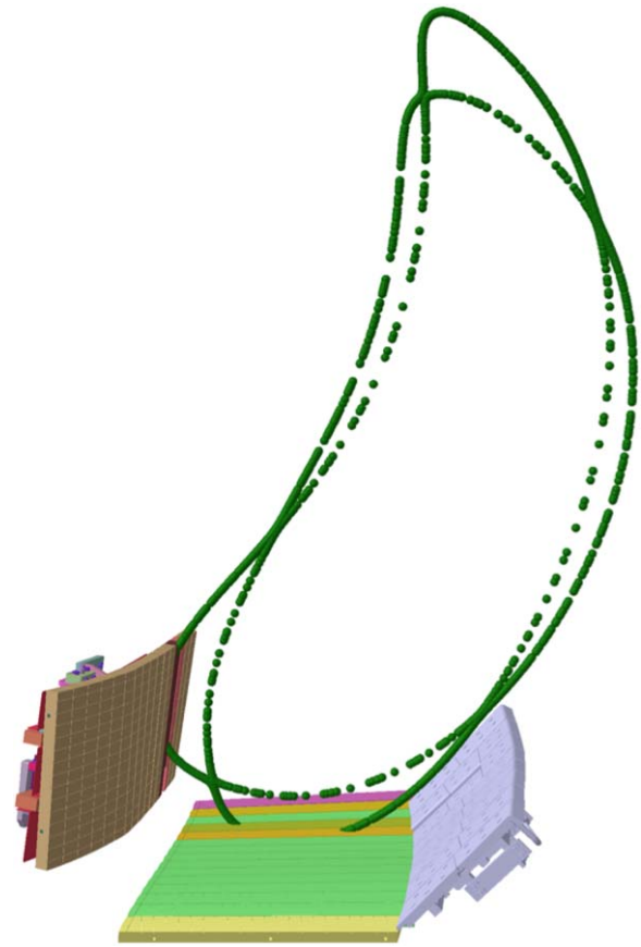
Figure 3. The island divertor concept is illustrated by displaying a Poincaré cross section in a CAD model of a divertor unit in W7-X. The island chain allows some physical separation between the edge of the confinement region and the region where the outflowing plasma hits the divertor plate.
