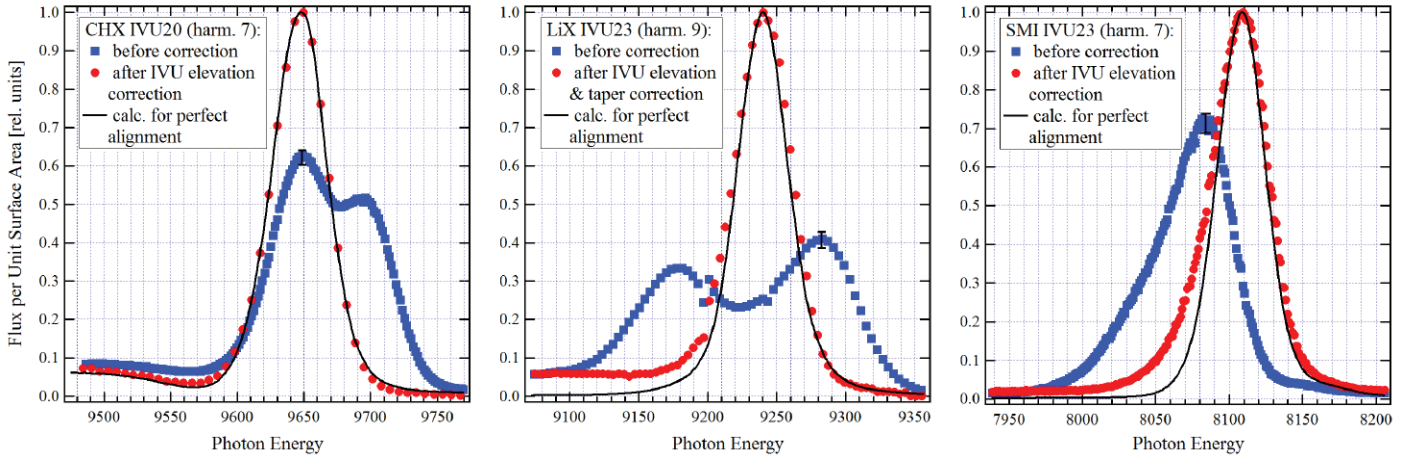
Figure 5: On-axis UR spectral flux per unit surface area measured before and after the spectrum-based alignment of IVU at three NSLS-II beamlines other than SRX: 3-m-long IVU20 at CHX (left), and 2.8-m-long IVU23 at LiX (middle) and SMI (right) beamlines. Solid lines in the graphs depict the corresponding calculated spectra at the assumption of perfect IVU alignment. All measurements and calculations were done at \epsilon_x \approx 0.9 nm and \sigma_E/E \approx 0.89 \times 10^{-3} , corresponding to the normal NSLS-II operation with the gaps of all three damping wigglers when closed.
