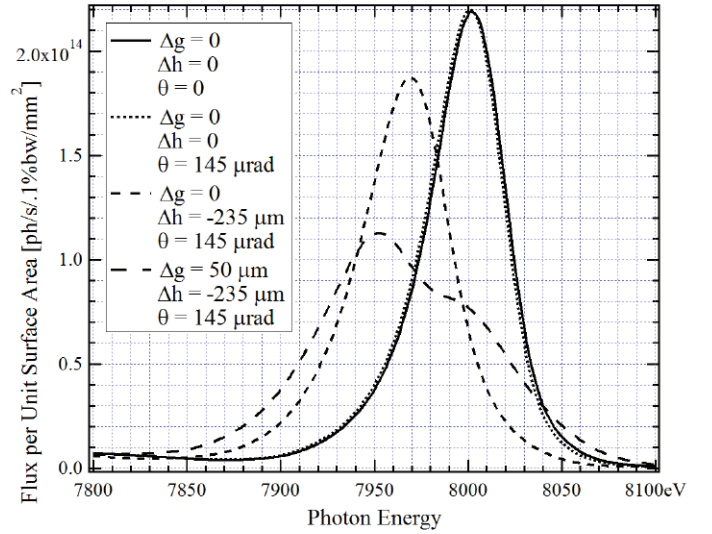
Figure 2: Calculated on-axis spectral flux per unit surface at 33 m observation distance at fifth harmonic of perfectly aligned IVU21 of SRX beamline (solid line) and for three misalignment cases (dotted/dashed lines).
