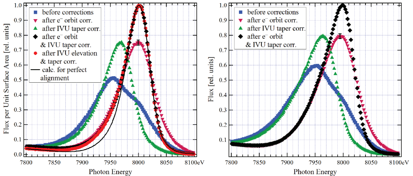
Figure 4: SRX IVU radiation spectra at fifth harmonic before and after applying electron orbit, undulator taper, and elevation corrections: on-axis spectral flux per unit surface area (left), and spectral flux within \sim 40 \times 40 \mu\text{rad}^2 aperture that is typically used for experiments at SRX (right).
