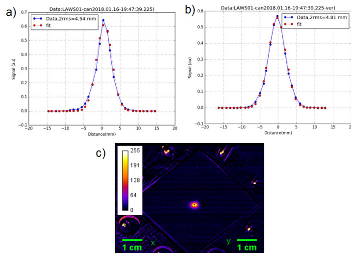
Figure 4. The beam profile at the end of linac a) horizontal and b) vertical, measured using a wire scanner; and (c) the beam profile at the end of the transport section using a gated CCD (LCTV4).
