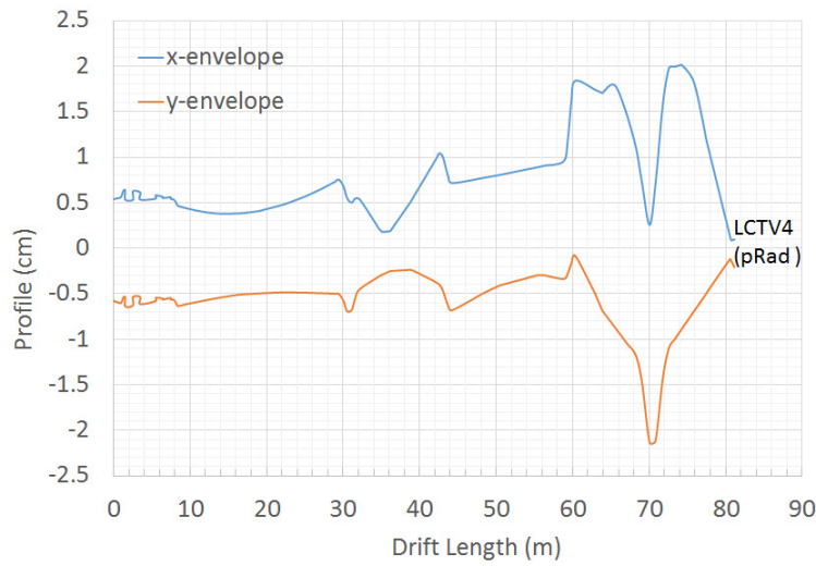
Figure 3. TRANSPORT calculated beam envelope.
