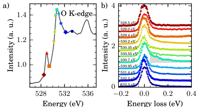
FIG. 2. a) O K-edge XAS taken with vertical polarization for 3/1 SL. Colored markers indicate energy positions where RIXS spectra were taken. b) RIXS spectra taken at several energies across the absorption edge. The low energy features appearing at the O K-edge white line, 530.7 eV, is highlighted in grey.
