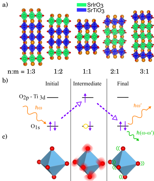
FIG. 1. a) Selected SL structures used for this investigation; the octahedral rotations are exaggerated for clarity. b) RIXS process for creating a phonon. c) Example octahedra during the RIXS scattering process, with the intermediate state hosting a poorly screened core hole distributed through the lattice that perturbs the O positions. The final state then involves one or more excited LO_4 phonon modes.
